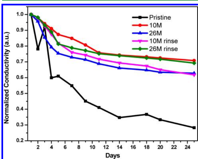
Figure 6. Conductivity stabilities of pristine and 10 and 26 M formic acid (both before and after rinsing) treated PEDOT:PSS films in the ambient atmosphere.
