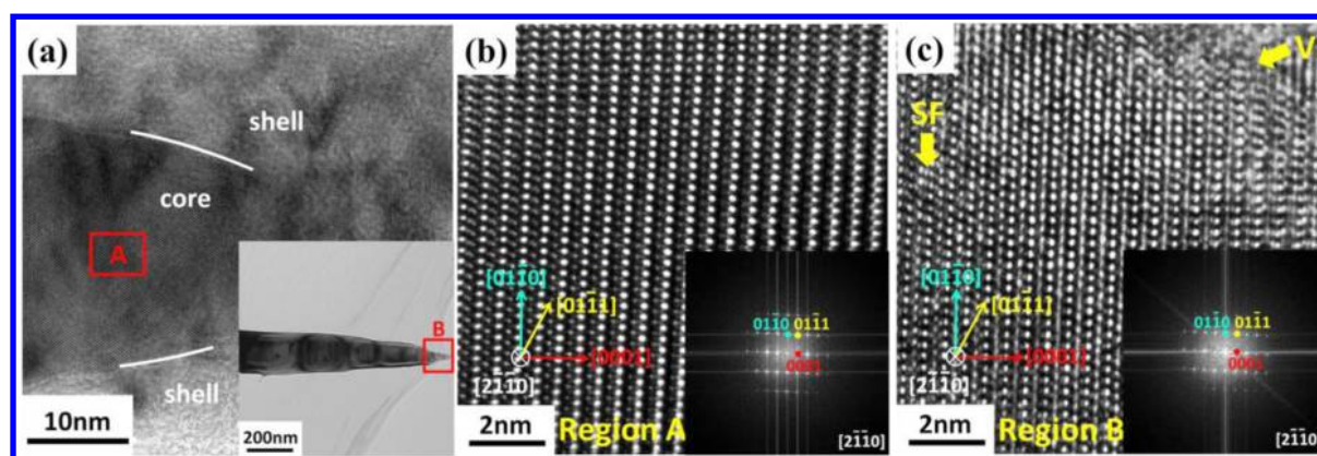
Figure 2. TEM images of a single SZO–GZO coaxial nanostructure: (a) high-magnification image; (inset) low-magnification image. HR-TEM images of (b) GZO core (region A in part a) and (c) SZO shell (region B in the inset of part a); (insets) their corresponding FFT diffraction patterns.
