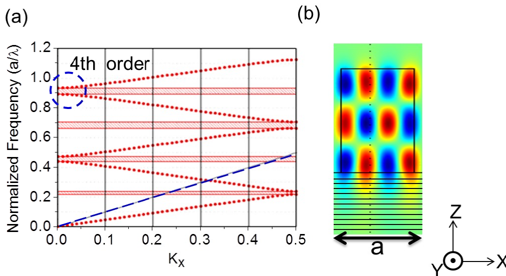
Figure 6 (a) The calculated band structure of GaN-based SELs using HCG using the PWE method. The blue dashed line represents the light line. The red dot lines represent the different order bands and the blue circle indicates the fourth order band. (b) The calculated mode pattern of GaN-based SELs using HCG using the finite element method. The parameter a is the grating period.
