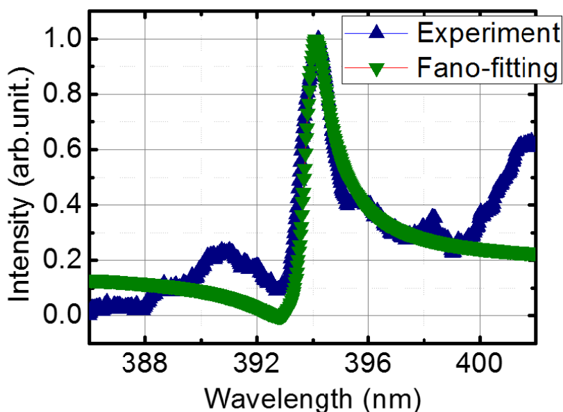
Figure 4 The PL spectra (navy curve) of GaN-based SELs using HCG when it was below the threshold condition. The olive curve shows the fitting result by Fano-resonance equation. The Q factor was calculated to be 394.
