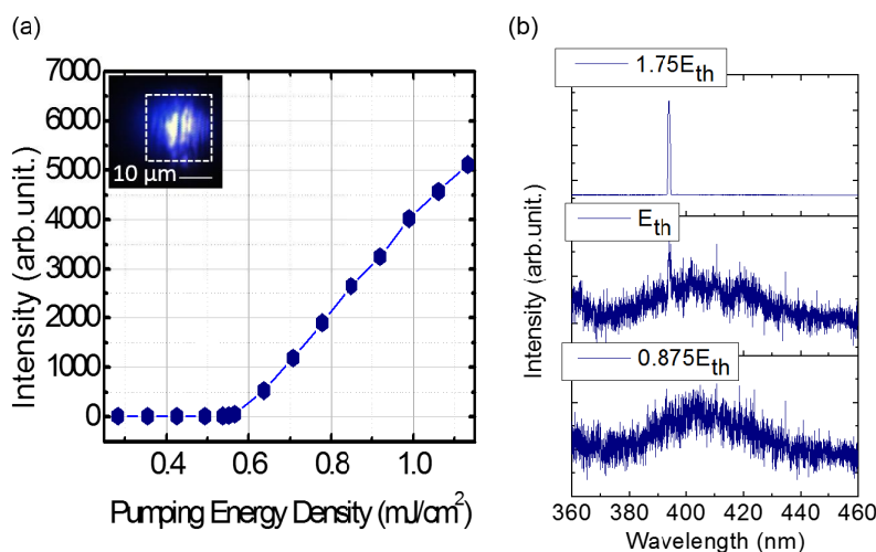
Figure 3 (a) The input-output characteristics of GaN-based SELs using HCG. The inset shows the CCD images when the GaN-based SELs using HCG was above the threshold condition. (b) The measured spectra with different pumping power of 0.875 E_{th} , E_{th} and 1.75 E_{th} . The full width at half maximum (FWHM) of lasing peak at 1.75 E_{th} is 0.88 nm.
