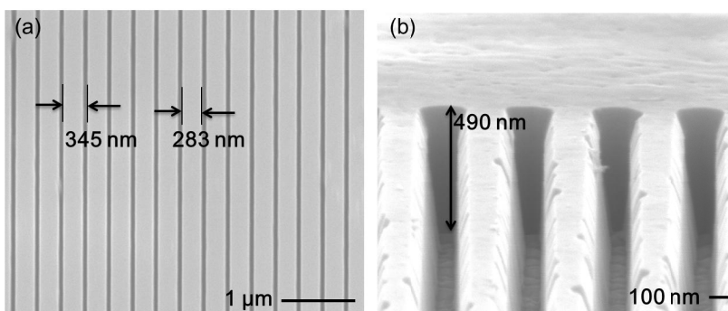
Figure 2 The (a) planar and (b) tilted angle SEM images of GaN-based SELs using HCG. The period, duty cycle and height of HCG were estimated to be 345 nm, 0.82 and 490 nm, respectively.
