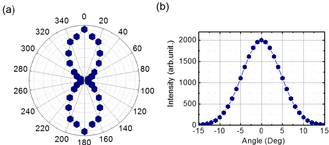
Figure 5 (a) The degree of polarization (DOP) and (b) the divergence angle of the GaN-based SELs using HCG when it was above the threshold condition. The detection direction was normal to the surface of the GaN-based SELs using HCG. The DOP and divergence angle were measured to be 73% and 12°, respectively.
