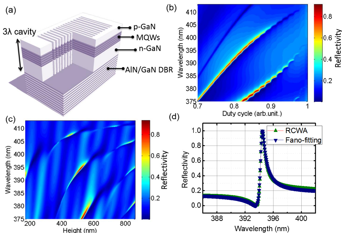
Figure 1 (a) Schemes of GaN-based SELs using HCG. (b) Reflectivity spectra mapping as a function of duty cycle (the grating width divided by the grating period). (c) Reflectivity spectra mapping versus grating height. (d) The reflectivity spectra for the grating with period: 345nm, filling factor: 0.82, grating height: 520 nm. The olive and navy curves show the simulation results by RCWA and fitting results by the Fano resonance equation.
