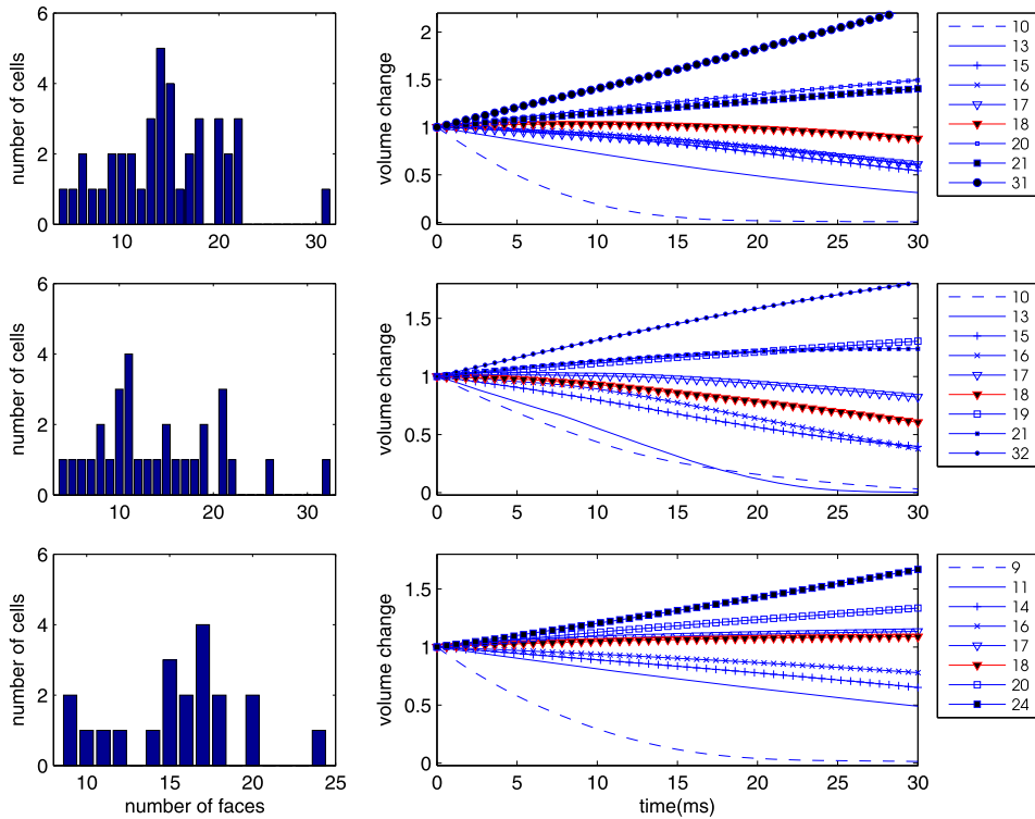
Fig. 16. The volume changes for the cells in the three different foams as functions of time. The volume changes are averaged over cells with the same numbers of faces. The left panels show the initial distribution of the number of cells versus the number of faces. The right panels show that the variation from the decrease to the increase of the cell volume occurs when the face number is between 17 and 19, i.e., F_0 = 18 \pm 1 .
