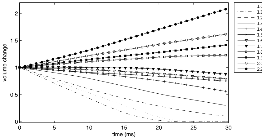
Fig. 15. The volume changes for all the cells in the foam as functions of time. The volume changes are averaged over cells with the same numbers of faces.
