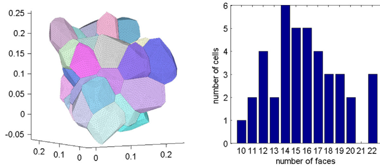
Fig. 12. The initial configuration of a general foam (left) and a histogram (right) showing the number of cells in the foam that have each of the different numbers of faces that actually occur in the foam (which vary from a minimum of 10 faces to a maximum of 22 faces). The configuration shown in the left panel was constructed by Voronoi tessellation of a periodic domain.
