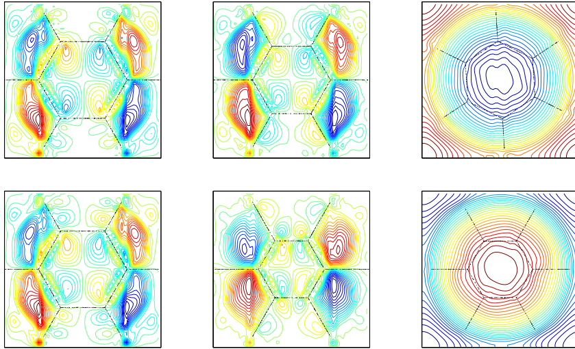
Fig. 10. The streamlines of the velocity field ( x and y components only) of the foam which has the number of radial planes n = 6 for three different cases: zero permeability in a stationary flow (left), M = 0.002 \text{ cm}^3/(\text{dyne s}) in a stationary flow (middle), and M = 0.002 \text{ cm}^3/(\text{dyne s}) in a dynamic flow (right). The velocity field is taken in the horizontal plane z = 0 , and the times are t = 24 \text{ ms} (top) and 40 \text{ ms} (bottom).
