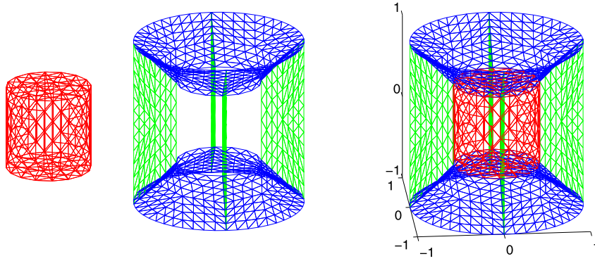
Fig. 4. Construction of an initial foam configuration. Left panel shows the “inner cell” of the foam (red), which is initially a circular cylinder with planar top and bottom. Middle panel shows n = 4 initially planar internal boundaries (green) of the foam that connect the inner cell to an outer rigid circular cylinder (not shown), and also two initially conical internal boundaries (blue) of the foam that connect the initially circular junction edges of the inner cell to the circular top and bottom of the outer rigid cylinder. The right panel shows all of the internal boundaries of the foam. In all three panels, the initial triangulation of these internal boundaries is shown. The triangulation in the figure is the one that is used with a 16 \times 16 \times 16 fluid grid, and is refined proportionally for use with finer grids. (For interpretation of the references to color in this figure legend, the reader is referred to the web version of this article.)
