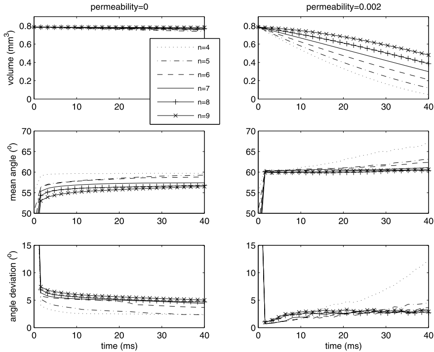
Fig. 8. The volume of the inner cell (top panels), the mean dihedral angle at the triple junctions (middle panels), and the root-mean-square deviation of the dihedral angles (bottom panels) as functions of time for the two permeability parameters: M = 0 (left panels) and M = 0.002 \text{ cm}^3/(\text{dynes}) (right panels).
