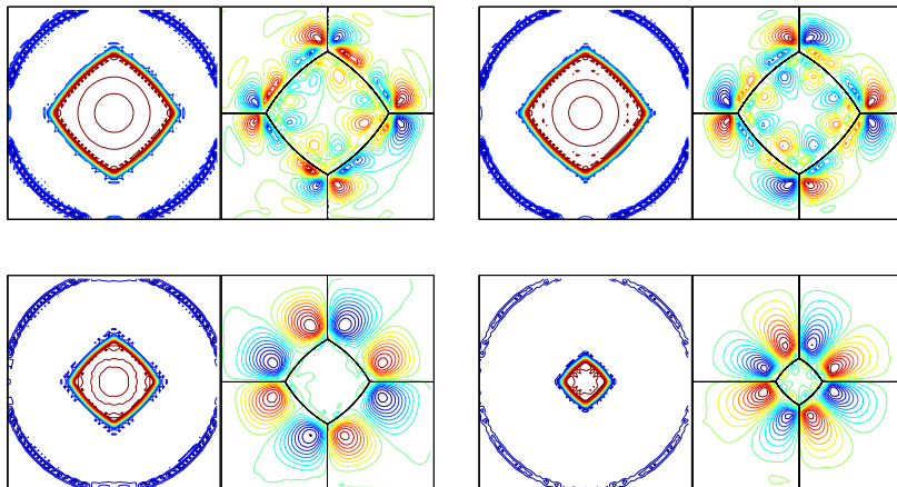
Fig. 6. Pressure contours (left panel of each pair of figures) and streamlines (right panel of each pair of figures) of the components u and v of the velocity fields on the middle horizontal plane z = 0 . The permeability is M = 0 (top panels) and M = 0.002 \text{ cm}^3/(\text{dyne s}) (bottom panels), and the times are 24 ms (left pairs) and 40 ms (right pairs). (For interpretation of the references to color in this figure, the reader is referred to the web version of this article.)
