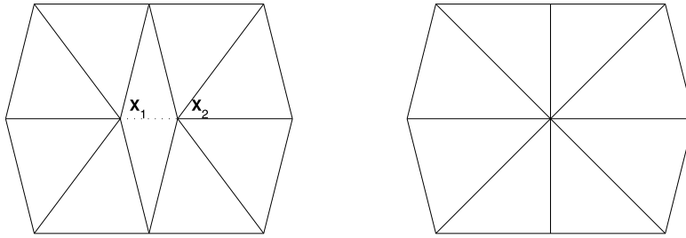
Fig. 3. Coarsening of edges and triangles. When the distance between two points \mathbf{X}_1 and \mathbf{X}_2 is less than h/5 (dotted line in the left panel), we delete both points and create in their place a new boundary point halfway between them. This deletes the edge that previously connected \mathbf{X}_1 and \mathbf{X}_2 , and it also deletes the two triangles which previously shared that edge. Any edge, other than the deleted edge, which previously had a vertex at \mathbf{X}_1 or \mathbf{X}_2 is now considered to have that vertex replaced by the new vertex, the location of which is (\mathbf{X}_1 + \mathbf{X}_2)/2 (right).
