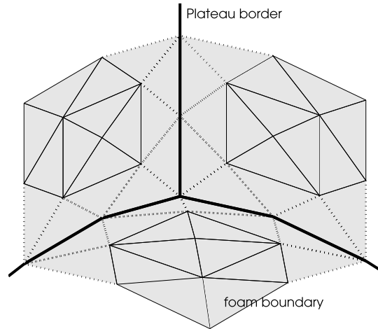
Fig. 1. Schematic figure of foam boundaries composed of three surfaces. The surfaces, which are modeled as triangular facets, meet at Plateau borders (bold lines). An edge of a triangle can be a part of the Plateau borders (bold lines, E_2 ), have only one vertex on a Plateau border (dotted lines, E_1 ), and have both vertices in the interior of some face (solid lines, E_0 ).
