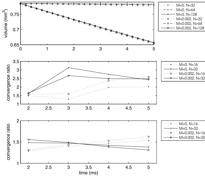
Fig. 7. The top panel shows the volume change of the inner cell in terms of time for each of the three mesh sizes ( N = 32, 64, and 128 ) and the two permeabilities ( M = 0 and 0.002 \text{ cm}^3/(\text{dyne s}) ), and the middle and bottom panels show the convergence ratios of the computed velocity field \mathbf{u}(\mathbf{x}, t) and pressure p(\mathbf{x}, t) of the fluid, respectively, for each of the two mesh sizes ( N = 16 and 32 ) and the two permeabilities ( M = 0 and 0.002 \text{ cm}^3/(\text{dyne s}) ). The convergence ratios for the velocity are near two (first order accuracy), and those for the pressure are around 1.3–1.5 (half-order accuracy).
