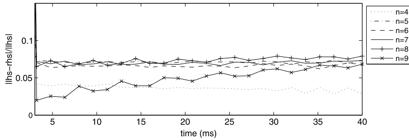
Fig. 9. Graphs of |lhs - rhs|/|lhs| in terms of time where lhs and rhs are defined in Eq. (27). The right- and left-hand sides of (27) are very close, which confirms the 3D generalized von Neumann relation (3) and thus (2) approximately.
