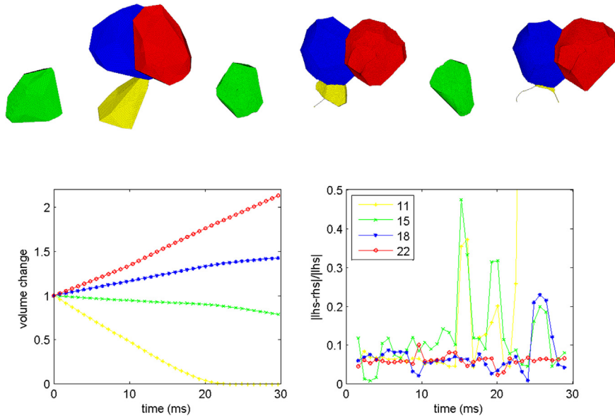
Fig. 14. Top: motion of cells with 11 faces (yellow one at the lower-right), 15 faces (green one at the lower-left), 18 faces (blue one at the upper-left), and 22 faces (red one at the upper-right) at some chosen times: t = 0, 12, and 24 from left to right. Bottom-left: volume change in time relative to the initial volumes of each of the four cells. Bottom-right: graph of |lhs - rhs|/|lhs| in terms of time where lhs and rhs are defined in (27). (For interpretation of the references to color in this figure legend, the reader is referred to the web version of this article.)
