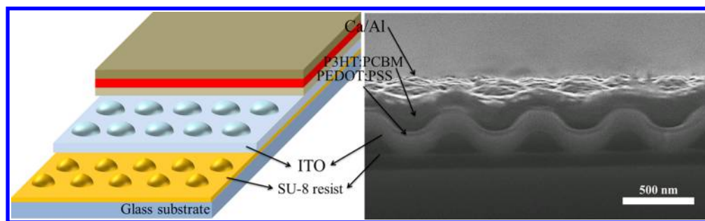
Figure 2. Schematic of the nanostructured substrate and the corresponding cross-section SEM image of the as prepared P3HT:PCBM solar cell.
