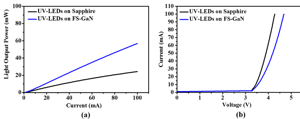
Fig. 7 (a) Light output as a function of forward current and (b) I-V characteristics for the UV-LEDs grown on FS-GaN and sapphire substrate. All data were obtained under continuous-wave (CW) operation.
