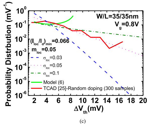
Fig. 9. Calculated \Delta V_{th} (green solid lines) headed and (nonsolid lines) tail distribution curves at (a) V_g = 0 , (b) V_g = 0.4 V, and (c) V_g = 0.8 V. Simulated (red solid lines) tail distributions due to random discrete dopants [25] are shown, along with calculated ones from several values of m_{loc} and \sigma_{loc} . Clearly, m_{loc} and \sigma_{loc} both must be reduced while entering into inversion regime, indicating that the underlying percolation paths electrically change, as well known in the field. V_d = 0.05 V in this paper.
