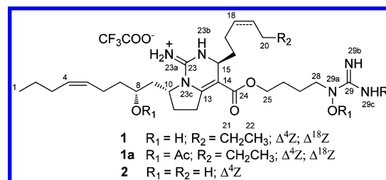
Figure 1. Structures of urupocidins A and B ( 1 and 2 ) and urupocidin A triacetate ( 1a ).
