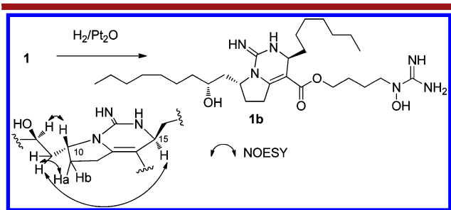
Figure 3. Hydrogenation of 1 and key NOEs correlations in 1b .
