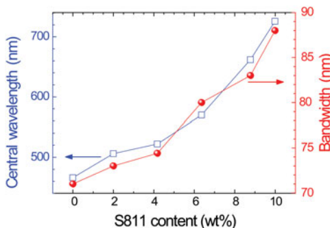
Figure 6. Both the central wavelength and reflection bandwidth varying with the S-811 concentration in CLC made of E7 doped with R-5011. The content of R-5011 in all cells is fixed at 2.87 \pm 0.15 wt%.
