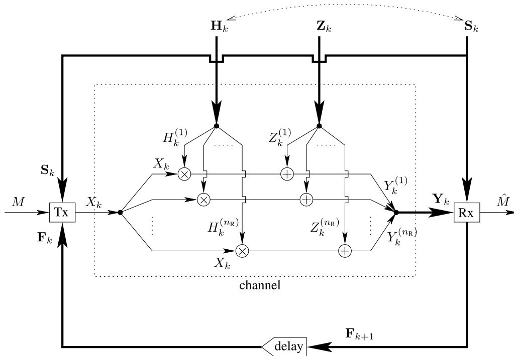
Fig. 1. SIMO fading channel with causal side-information at both transmitter and receiver and a noiseless causal feedback link from the receiver back to the transmitter.
