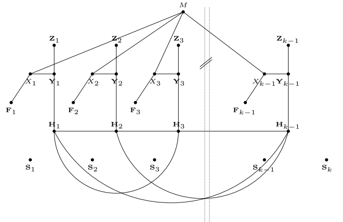
Fig. 3. The causally relevant subgraph of (303) showing the independence of M and S_k when conditioned on (Y_1^{k-1}, S_1^{k-1}) .
