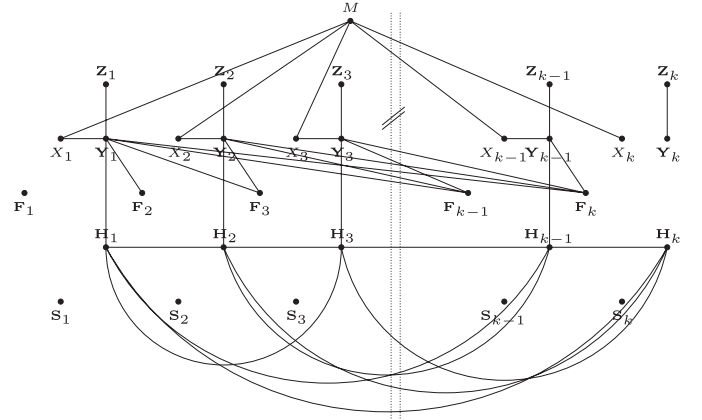
Fig. 12. The causally relevant subgraph of (303) showing the independence of \mathbf{Y}_k and \mathbf{H}_1^{k-1} when conditioned on (X_k, \mathbf{H}_k, \mathbf{S}_1^k, \mathbf{F}_1^k) .
