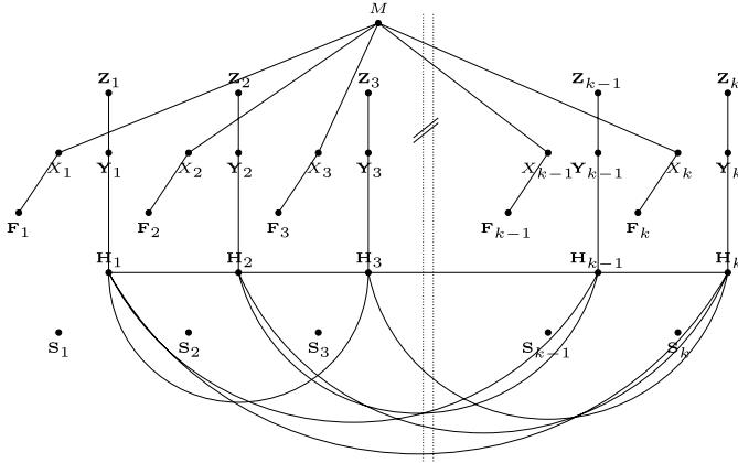
Fig. 9. The causally relevant subgraph of (303) showing the independence of \mathbf{Y}_k and M when conditioned on (\mathbf{Y}_1^{k-1}, X_1^k, \mathbf{S}_1^k) .
