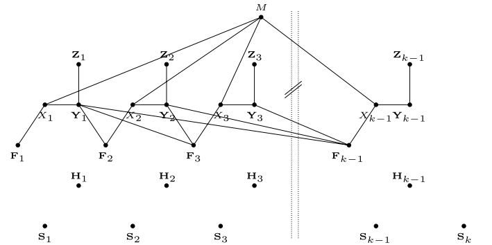
Fig. 8. The causally relevant subgraph of (303) showing the independence of \mathbf{S}_k and (X_1^{k-1}, \mathbf{Y}_1^{k-1}) when conditioned on (\mathbf{H}_1^{k-1}, \mathbf{S}_1^{k-1}) .
