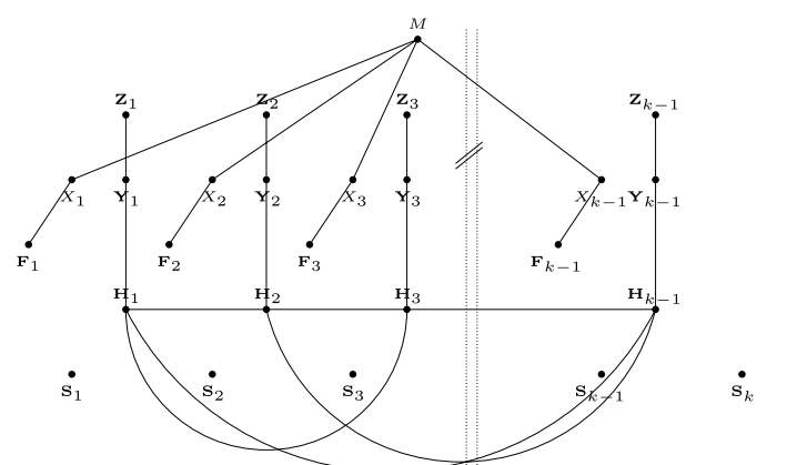
Fig. 7. The causally relevant subgraph of (303) showing the independence of \mathbf{S}_k and M when conditioned on (\mathbf{Y}_1^{k-1}, X_1^{k-1}, \mathbf{S}_1^{k-1}) .
