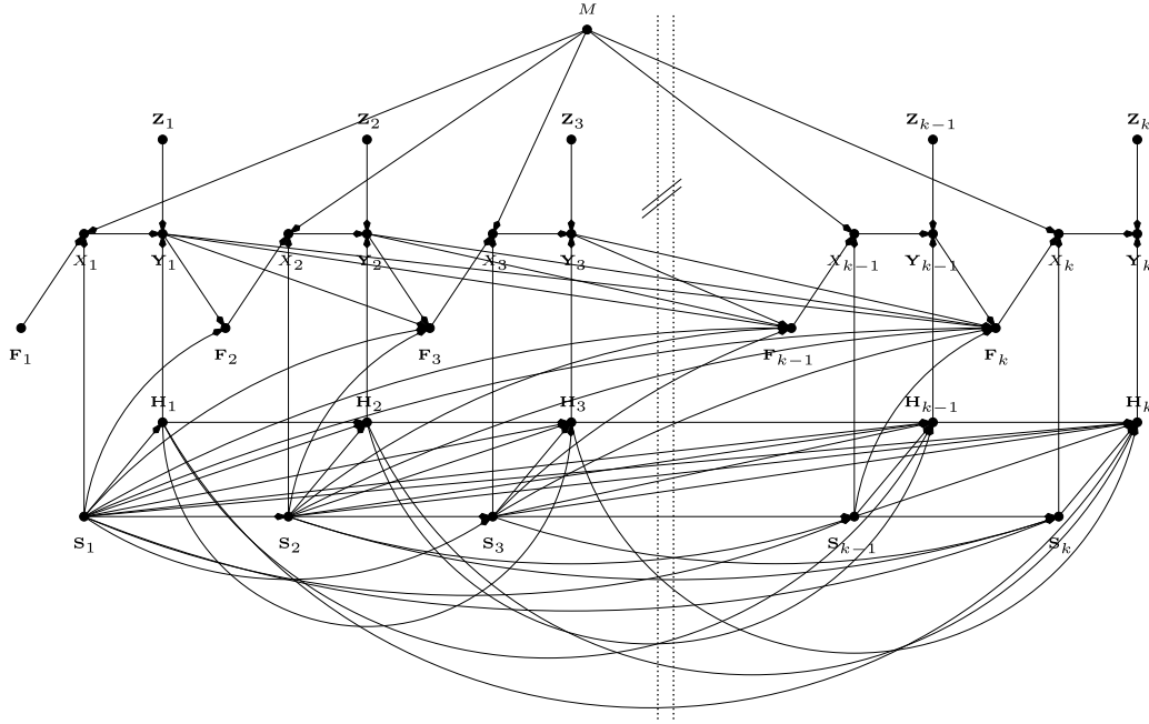
Fig. 2. The causality graph of the causal-order expansion given in (303).
