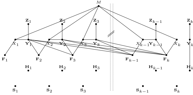
Fig. 4. The causally relevant subgraph of (303) showing the independence of (M, \mathbf{Y}_1^{k-1}) and \mathbf{Y}_k when conditioned on (X_k, \mathbf{H}_1^{k-1}, \mathbf{S}_1^k) .
