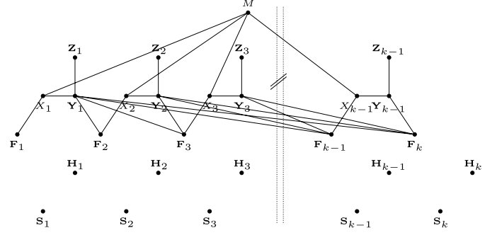
Fig. 13. The causally relevant subgraph of (303) showing the independence of \mathbf{H}_k and \mathbf{F}_1^k when conditioned on (\mathbf{H}_1^{k-1}, \mathbf{S}_1^k) .
