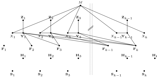
Fig. 11. The causally relevant subgraph of (303) showing the independence of X_k and \mathbf{H}_k when conditioned on (\mathbf{H}_1^{k-1}, \mathbf{S}_1^k, \mathbf{F}_1^k) .
