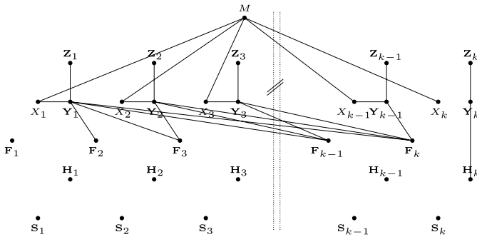
Fig. 10. The causally relevant subgraph of (303) showing the independence of \mathbf{Y}_k and (X_1^{k-1}, \mathbf{Y}_1^{k-1}) when conditioned on (X_k, \mathbf{H}_1^{k-1}, \mathbf{S}_1^k, \mathbf{F}_1^k) .
