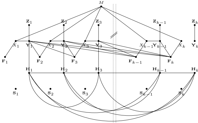
Fig. 5. The causally relevant subgraph of (303) showing the independence of \mathbf{Y}_k and \mathbf{H}_1^{k-1} when conditioned on (X_k, \mathbf{H}_k, \mathbf{S}_1^k) .
