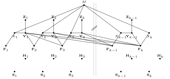
Fig. 6. The causally relevant subgraph of (303) showing the independence of X_k and \mathbf{H}_k when conditioned on (\mathbf{H}_1^{k-1}, \mathbf{S}_1^k) .
