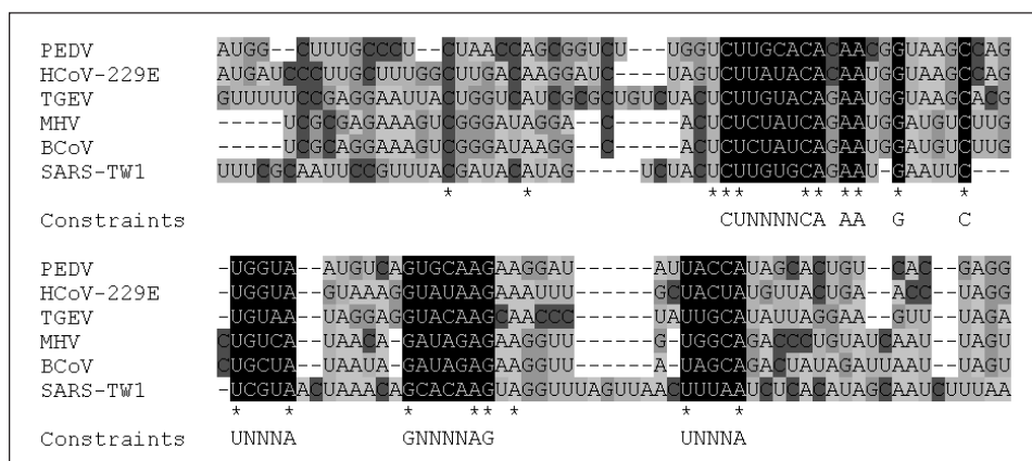
Fig. 4. The partial display of the resulting CMSA of MuSiC-ME by aligning the sequences of SARS-TW1 3'-UTR with those of other five coronaviruses.
