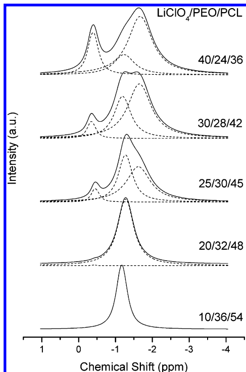
Figure 9. Solid-state 7 Li proton-decoupled MAS NMR spectra of ternary blends of LiClO 4 /PEO/PCL having a fixed PEO/PCL ratio of 40/60.
