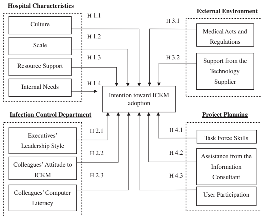
Fig. 1. Research framework.
