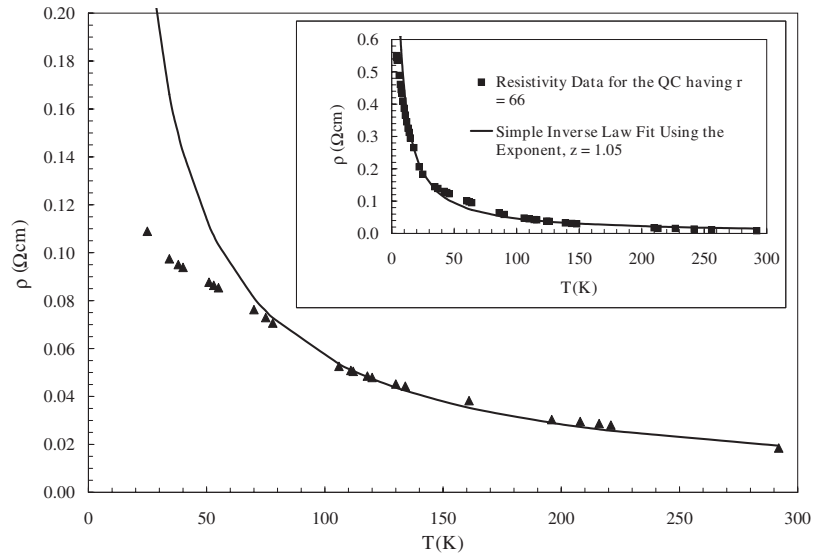
Figure 1. High temperature resistivity data (triangles) for an AlPdRe QC having r_T = 9.3 . The fit (solid curve) is a simple inverse temperature law where \rho(T) = 5.68/T^{1.00} in \Omega\text{ cm} . The inset shows data (squares) for the QC having r_T = 66 ; the fit (solid curve) is \rho(T) = 5.88/T^{1.05} in \Omega\text{ cm} .
