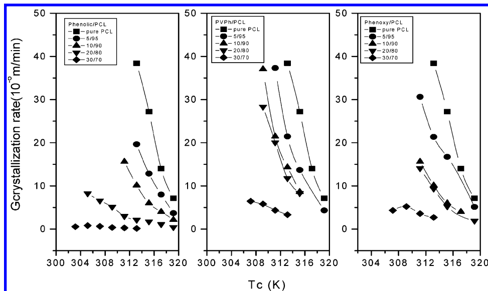
Figure 6. Radial growth rate ( G ) as a function of T_c for phenolic/PCL, PVPh/PCL, and phenoxy/PCL blends.
