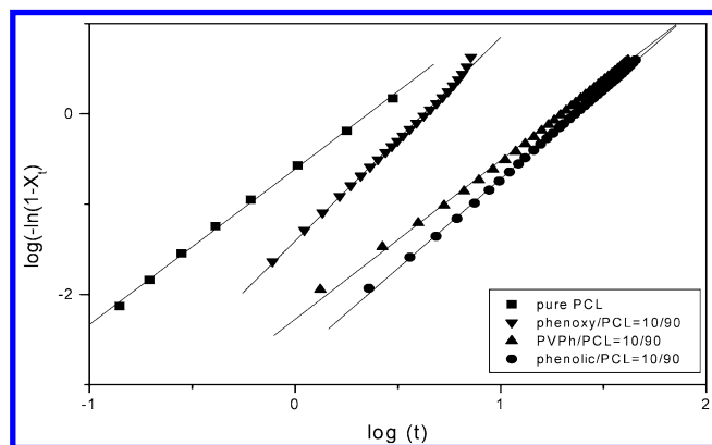
Figure 3. Avrami plot for pure PCL, phenolic/PCL = 10/90, PVPh/PCL = 10/90, and phenoxy/PCL = 10/90 blends at 40 °C.
