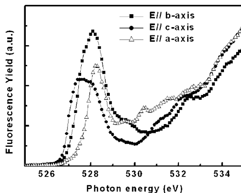
Fig. 2. Comparison of the O 1s absorption spectra of (100) oriented YBCO thin films for polarization E\parallel a -, E\parallel b - and E\parallel c -axes.
