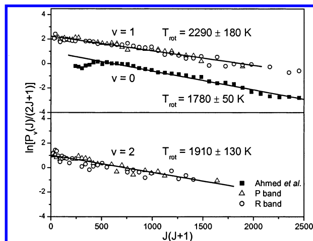
Figure 3. Semilogarithmic plots of relative rotational populations of CO ( v' = 1 and 2) upon photolysis of (\text{CICO})_2 at 248 nm. Symbols \Delta are from P lines and \circ are from R lines; data reported by Ahmed et al. (ref 6; symbol \blacksquare ) for v = 0 are also shown (displaced downward) for comparison. Solid lines represent least-squares fits.
