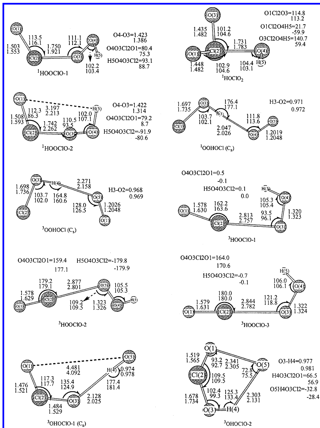
Figure 1. Optimized geometries of the intermediates (lengths in Å and angles in degrees). The top numbers were optimized at the B3LYP/6-311+G(3df,2p) level; the bottom numbers were optimized at the B3LYP/6-311G(d,p) level.
