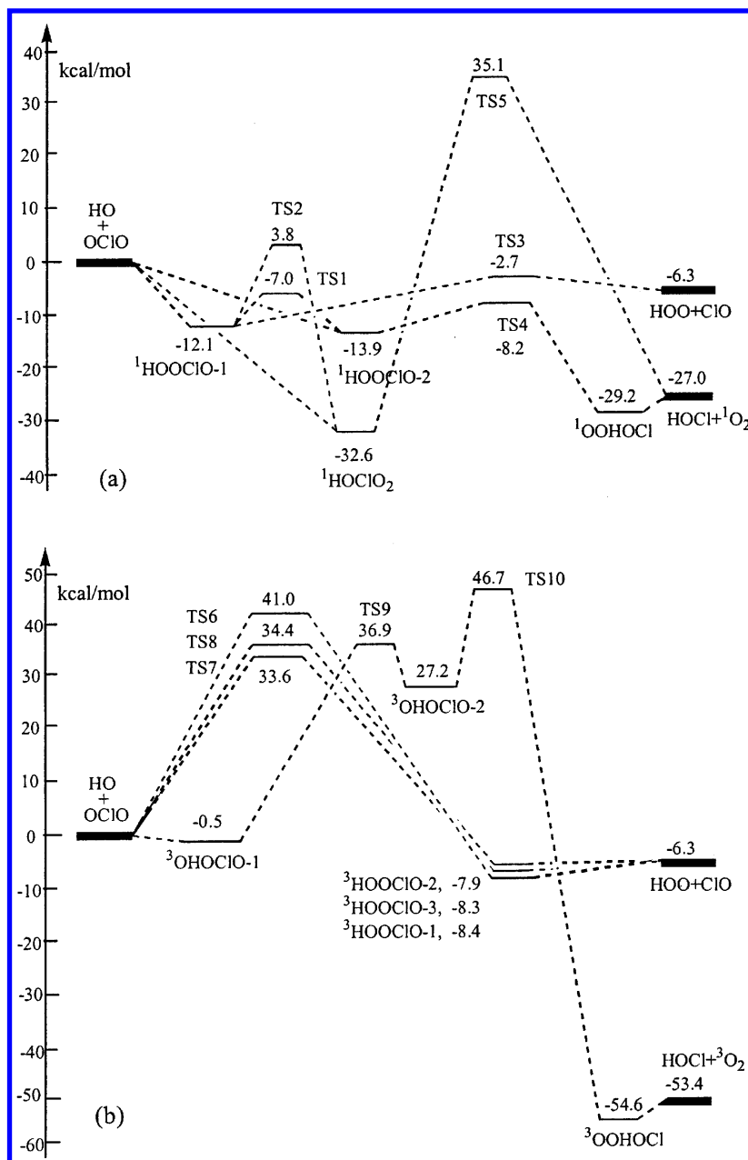
Figure 3. Schematic energy diagram of the OH + OClO system calculated by means of the G2M(CC2) method with the geometry parameters optimized at the B3LYP/6-311+G(3df,2p) level.
