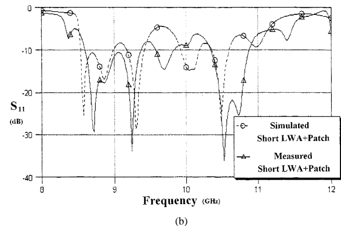
Fig. 2. (a), (b): Simulated and measured S_{11} parameters of the conventional short LWA (two wavelengths) with the open end and the proposed LWA integrated with the two-element phased array.
