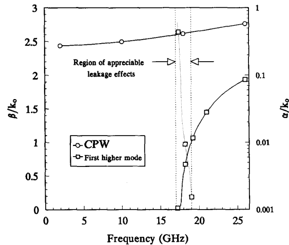
Fig. 10. Dispersion characteristics of the modified FW-CBCPW as shown in Fig. 8. -o- Normalized phase constants of CPW mode; -□- Normalized phase constants of the first higher order mode; -.- Normalized leaky constants of the first higher order mode.
