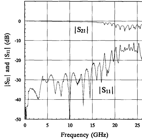
Fig. 9. The measured transmission ( |S_{21}| ) and reflection ( |S_{11}| ) characteristics of the modified FW-CBCPW through line of Fig. 8. The through line length L is equal to 38.1 mm.
