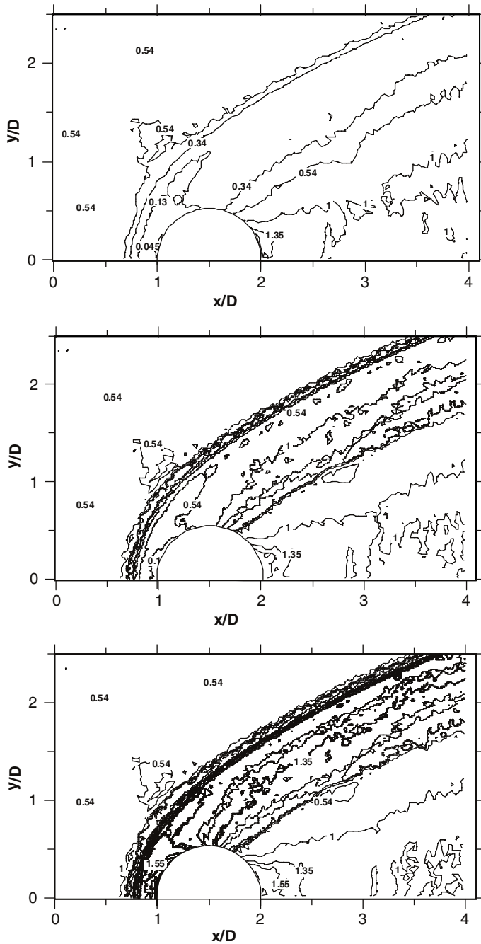
Figure 11. Evolution of local cell Knudsen number for a hypersonic flow over a cylinder; (a) initial (b) level 2 (c) level 5 ( Kn_\infty = 0.025 ; Kn_{cc} = 1 ; \phi_0 = 1.05 ).
