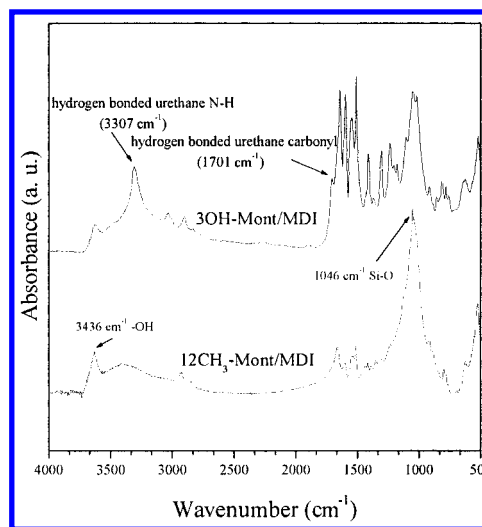
Figure 4. Fourier transform infrared spectra of 12CH 3 -Mont/MDI and 3OH-Mont/MDI.
