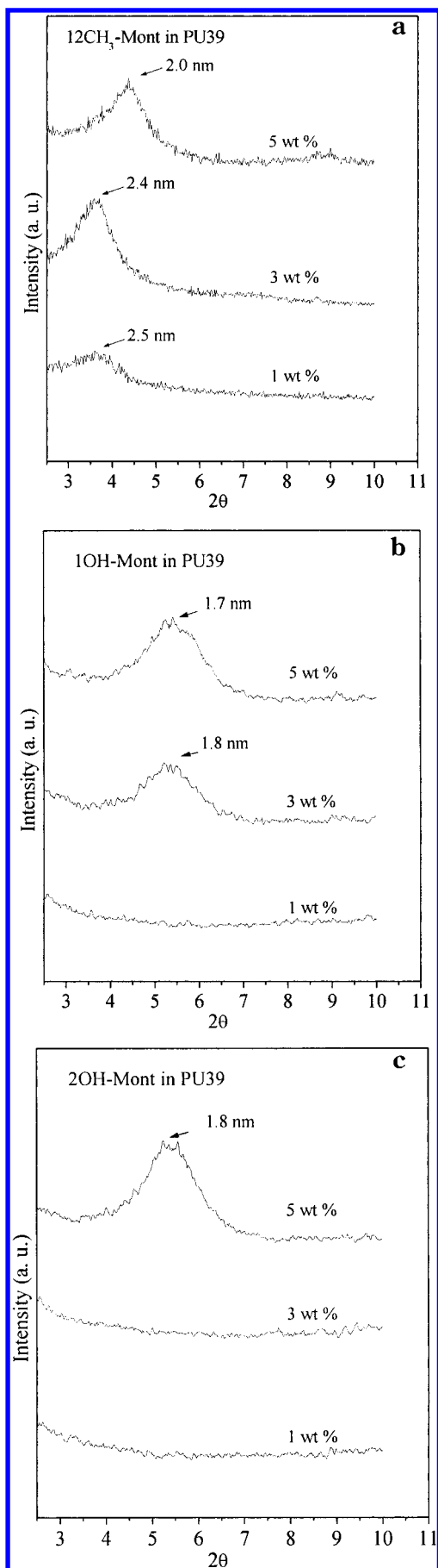
Figure 3. Wide-angle X-ray diffraction curves of PU39 containing 1, 3, and 5 wt % (a) 12CH 3 -Mont, (b) 1OH-Mont, and (c) 2OH-Mont.
