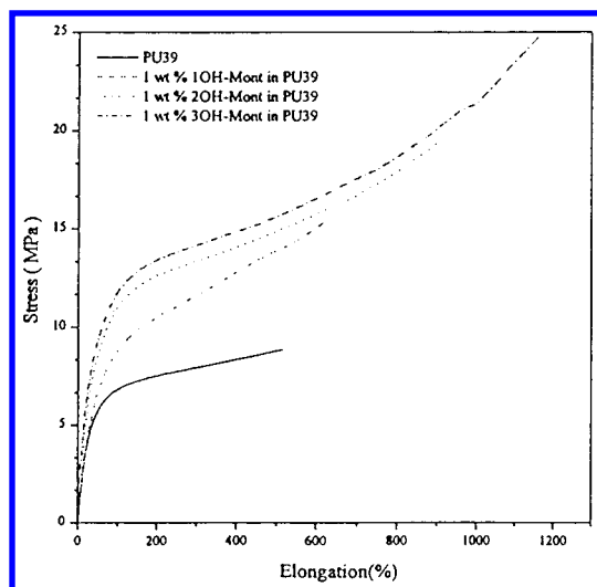
Figure 7. Stress-strain curves of PU39 containing 1 wt % tethered-Mont.
