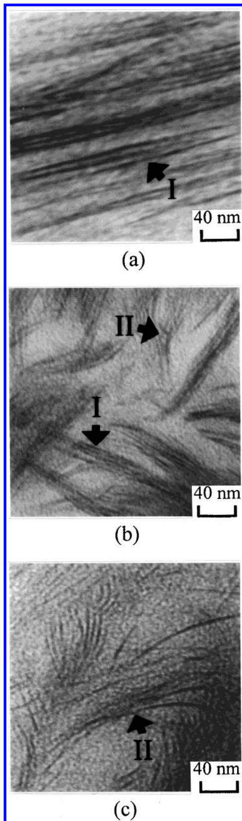
Figure 5. Transmission electron microscopy micrographs of the cross-sectional views of PU39 containing (a) 1 wt % 1OH-Mont (b) 1 wt % 2OH-Mont, and (c) 1 wt % 3OH-Mont: (I) indicated intercalated structure; (II) indicated exfoliated structure.
