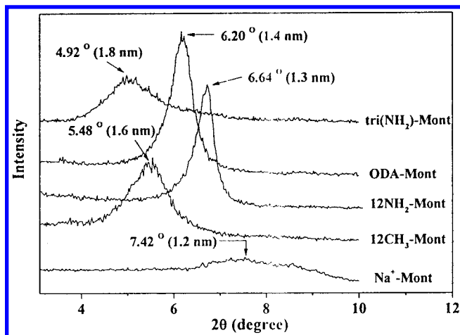
Figure 2. X-ray diffraction curves of pure montmorillonite and of swelling-agent-modified montmorillonite.
