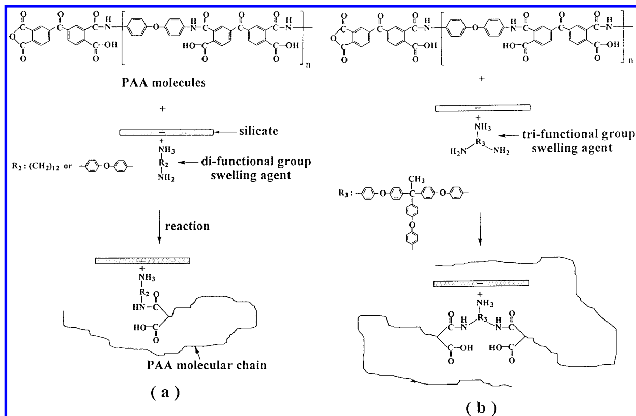
Figure 1. Schematic drawings of (a) difunctional group ( -\text{NH}_2 ) swelling agent and (b) trifunctional group swelling agent for intercalating layered silicates and reacting with poly(amic acid) molecules.
