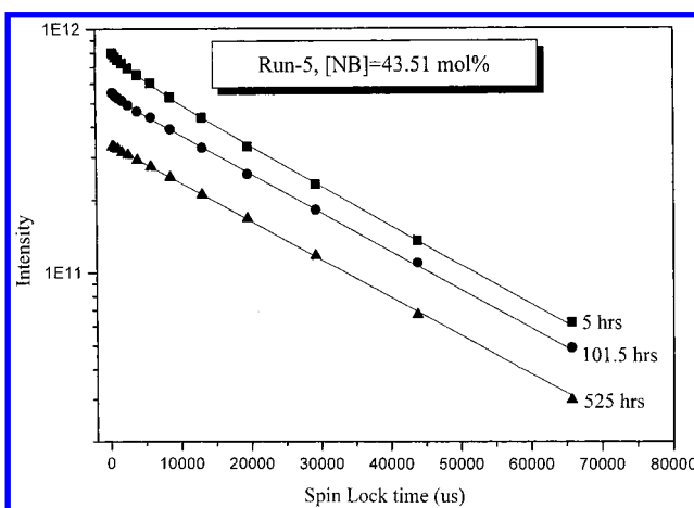
Figure 6. Semilog decay curve of COC T_{1p}^H relaxation experiment with varying annealing time.
