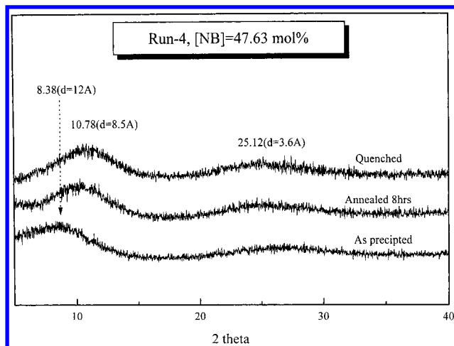
Figure 5. Synchrotron radiation powder X-ray diffraction of run 4 (a) before and (b) after extensive annealing.
