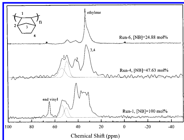
Figure 3. Solid-state ^{13}\text{C} NMR CP/MAS spectra for sample 1, run 4 and run 6. The assignment is labeled in the inset. The dashed curve represents the best fit with two Gaussian components.
