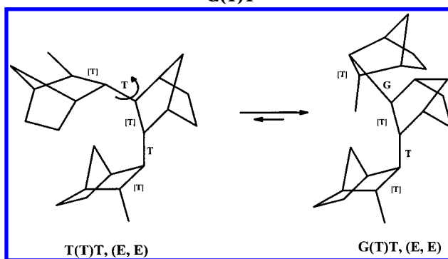
Scheme 5. Conformation Interconversion of T(T)T to G(T)T
