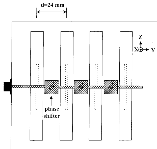
Fig. 1. Schematic of the aperture coupled linear 4 \times 1 dual-beam 2-D scanning microstrip leaky-wave antenna array.
