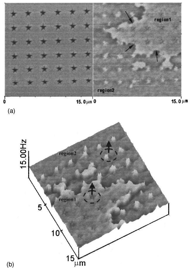
FIG. 4. For the Dy_{22}(Fe_{80}Co_{20})_{78} sample, (a) the left half shows the measured star-shaped topography images; the right half is simultaneously measured magnetic domain image; (b) 3D zoom-in image of right half of (a).
