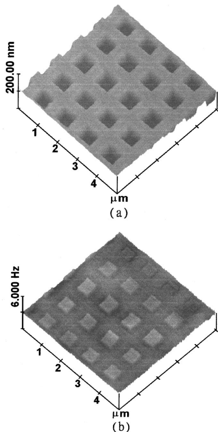
FIG. 3. (a) Displays the patterned topography of 500 nm×500 nm square holes with 1000 nm period; (b) is the corresponding pinned domains within holes.
