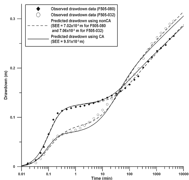
Fig. 4 The drawdown curves predicted by Neuman's solution (Neuman 1974) with parameters determined from nonCA and CA for wells F505-032 and F505-080
