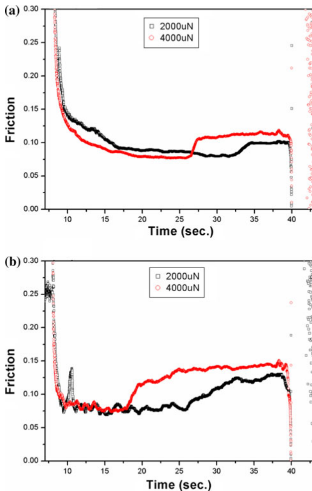
Fig. 2 Typical profiles of the coefficient of friction ( \mu ) plotted with respect to the scratch duration at ramped loads of 2,000 and 4,000 \mu\text{N} for GaN films on a c-axis and b a-axis sapphire substrates
