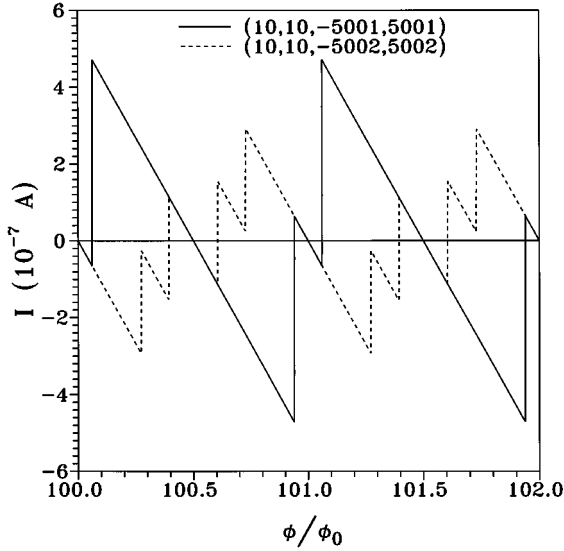
FIG. 6. Same plot as Fig. 3, but the Zeeman splitting is taken into account.
