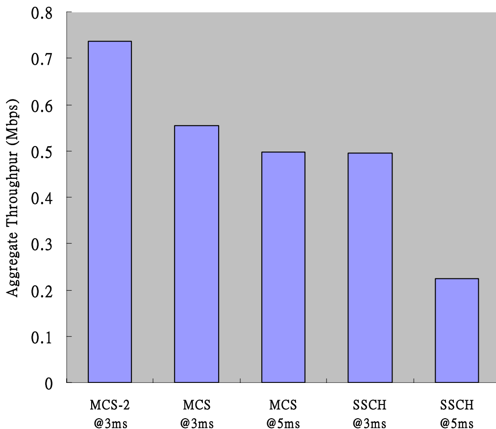
圖 5-4 Impact of switching latency
