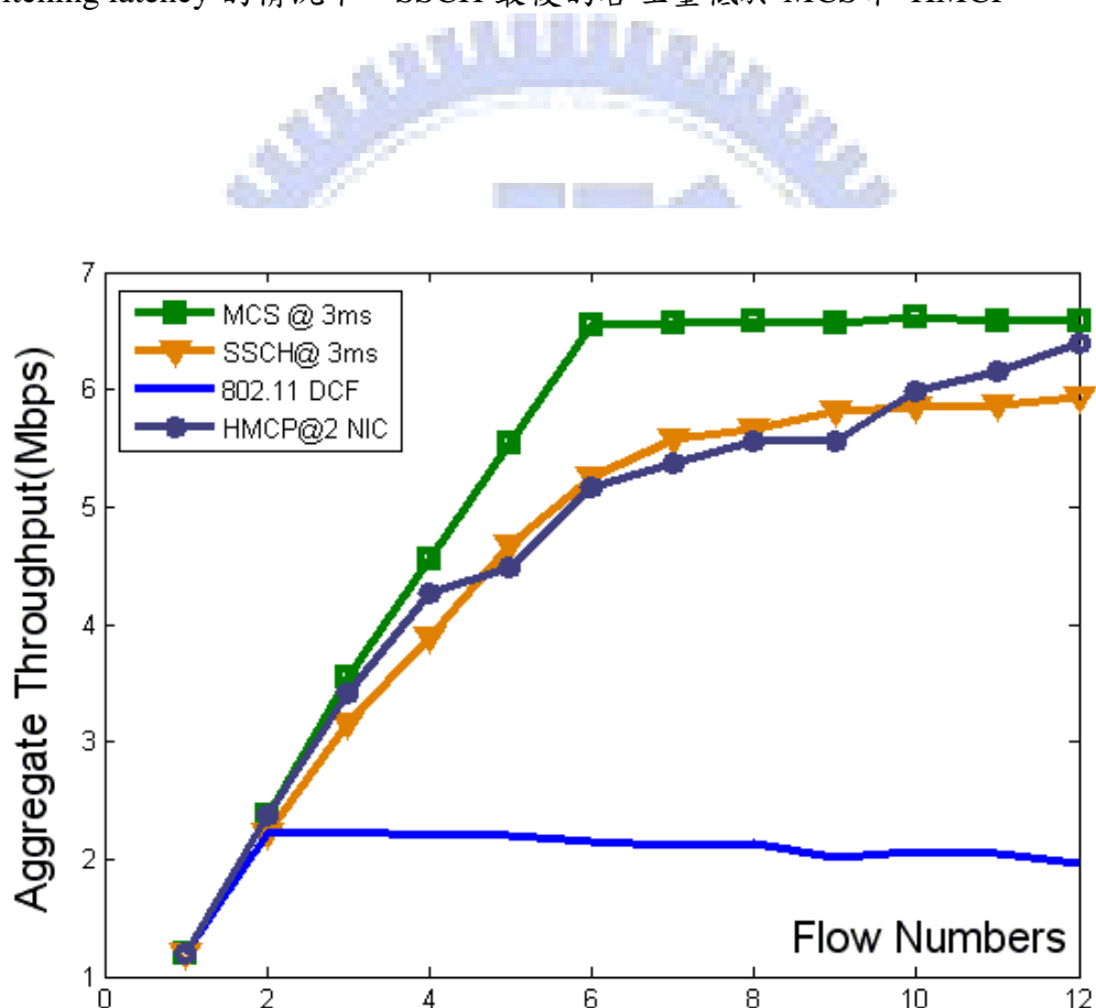
圖 5-3 Impact of unbalanced channel loading
