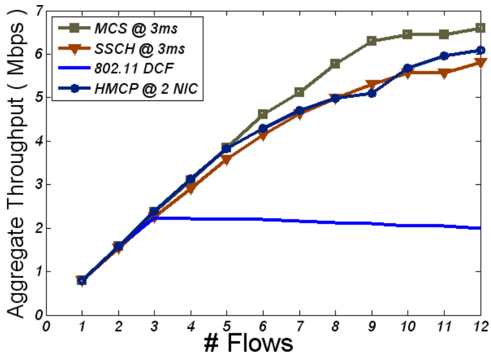
圖 5-2 Performance comparison v.s. number of UDP flows
