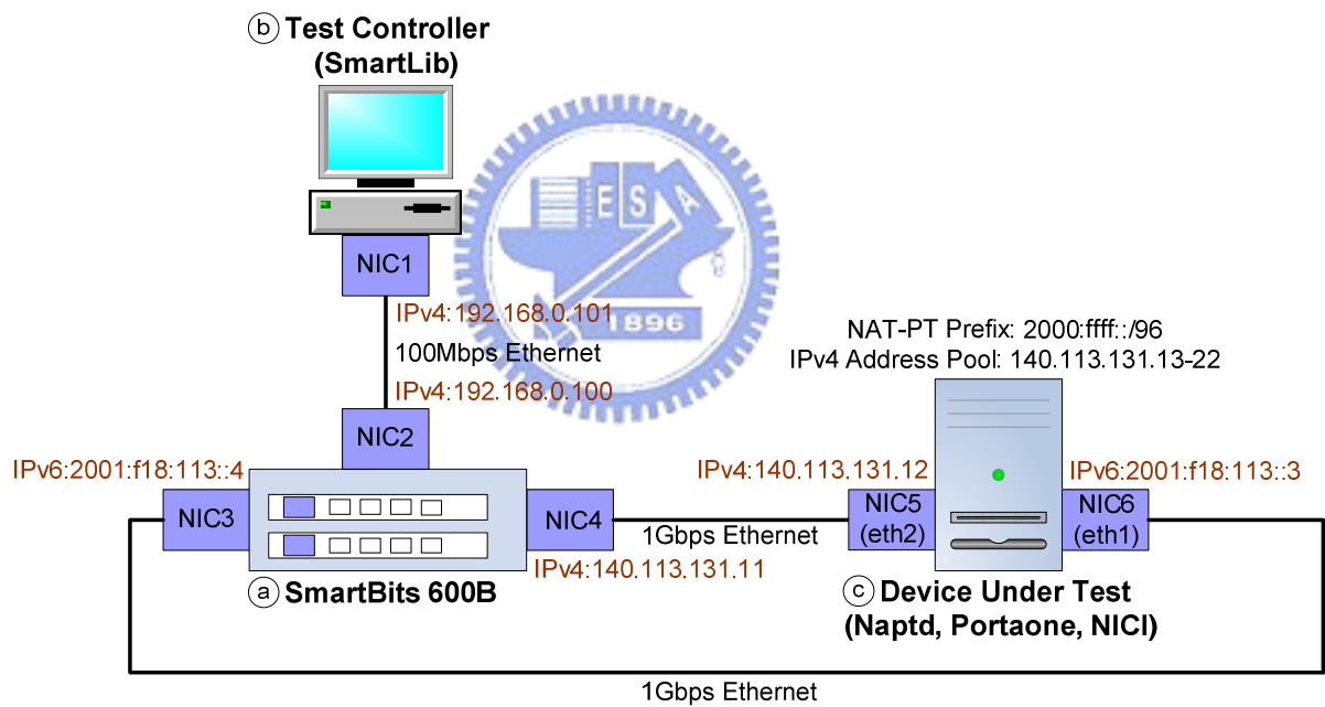
Fig. 7. The Test Environment for IPv4-IPv6 Translation
