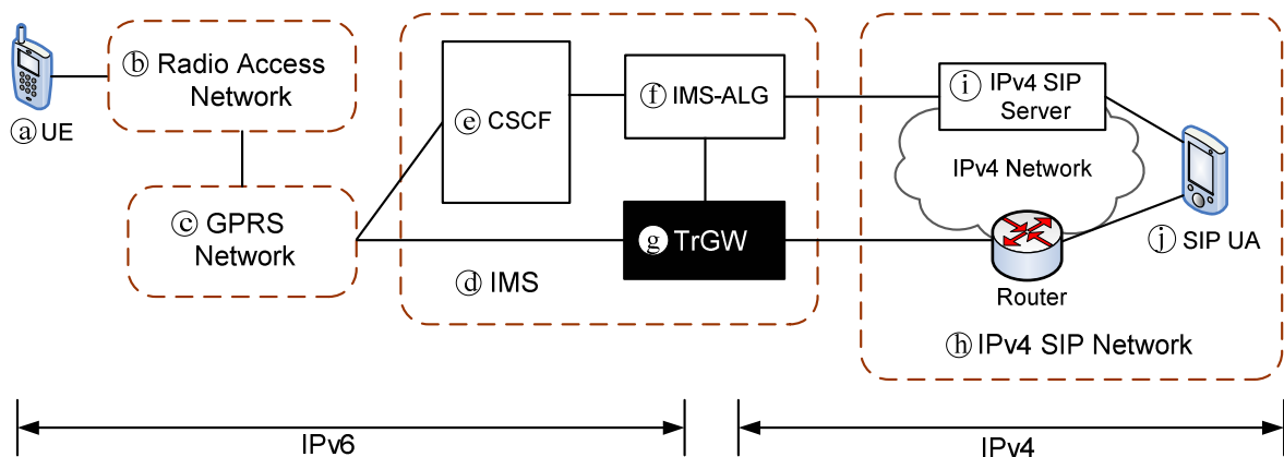
Fig. 1. Interworking between the IPv6-based IMS and the IPv4 VoIP networks
