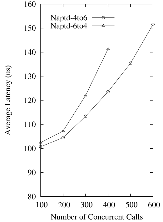
(b) Naptd IPv4-to-IPV6 and IPV6-to-IPV4
