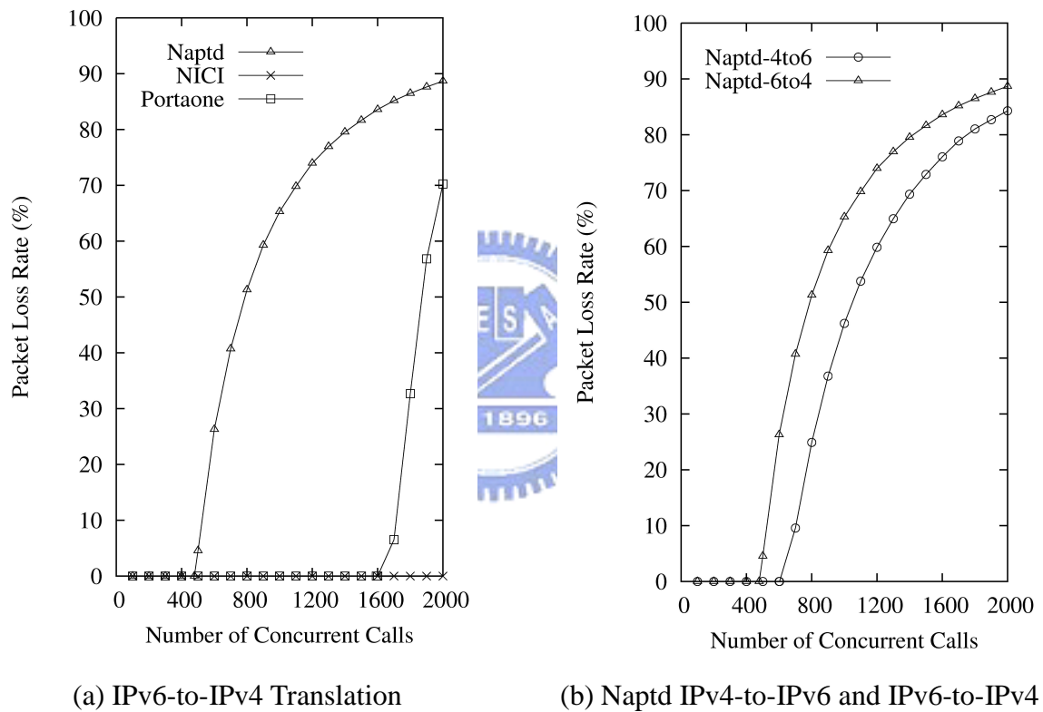
Fig. 8. The Packet Loss Rate
