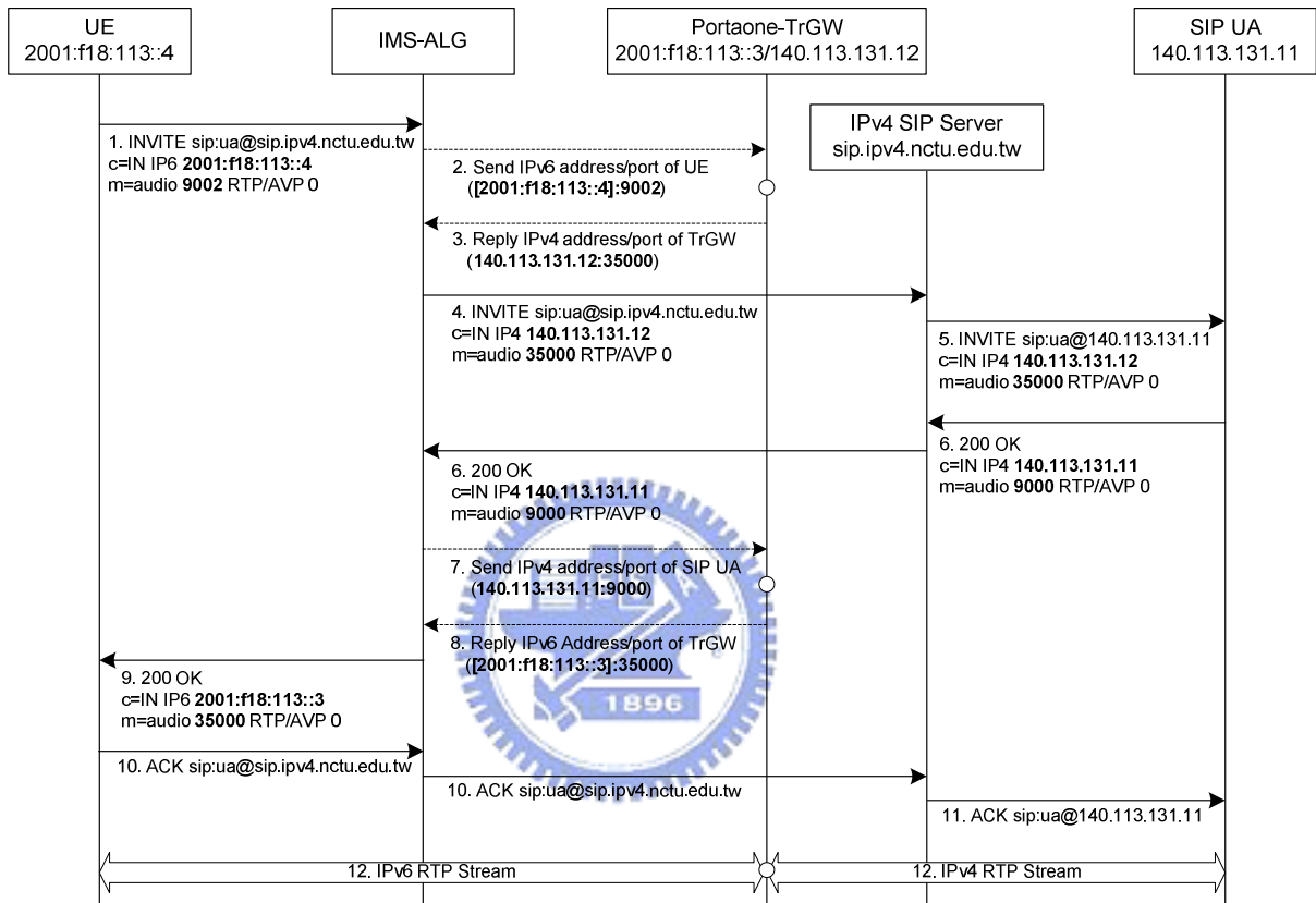
Fig. 4. SIP message flow with Portaone-TrGW
