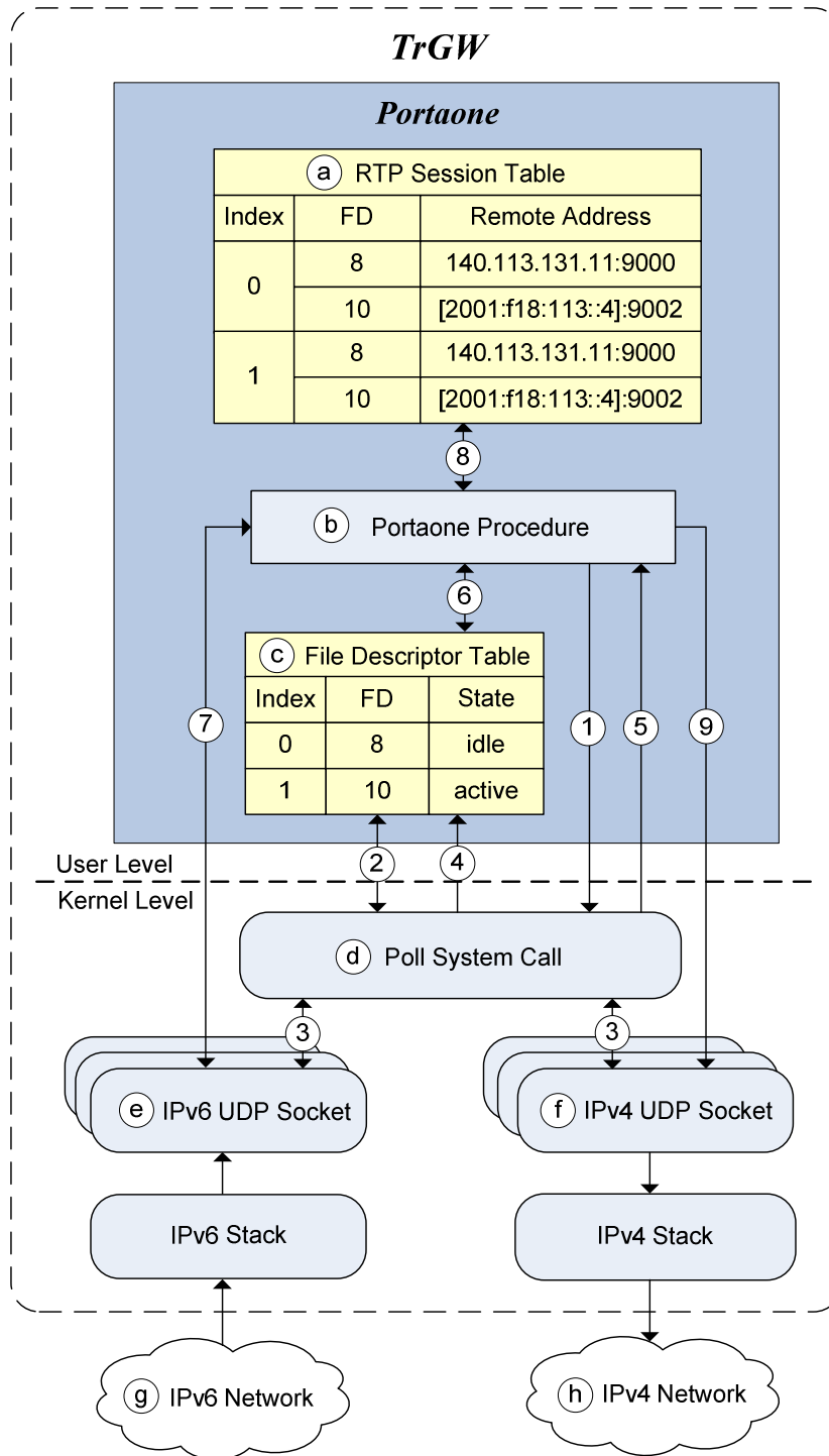
Fig. 5. Portaone-TrGW Architecture
