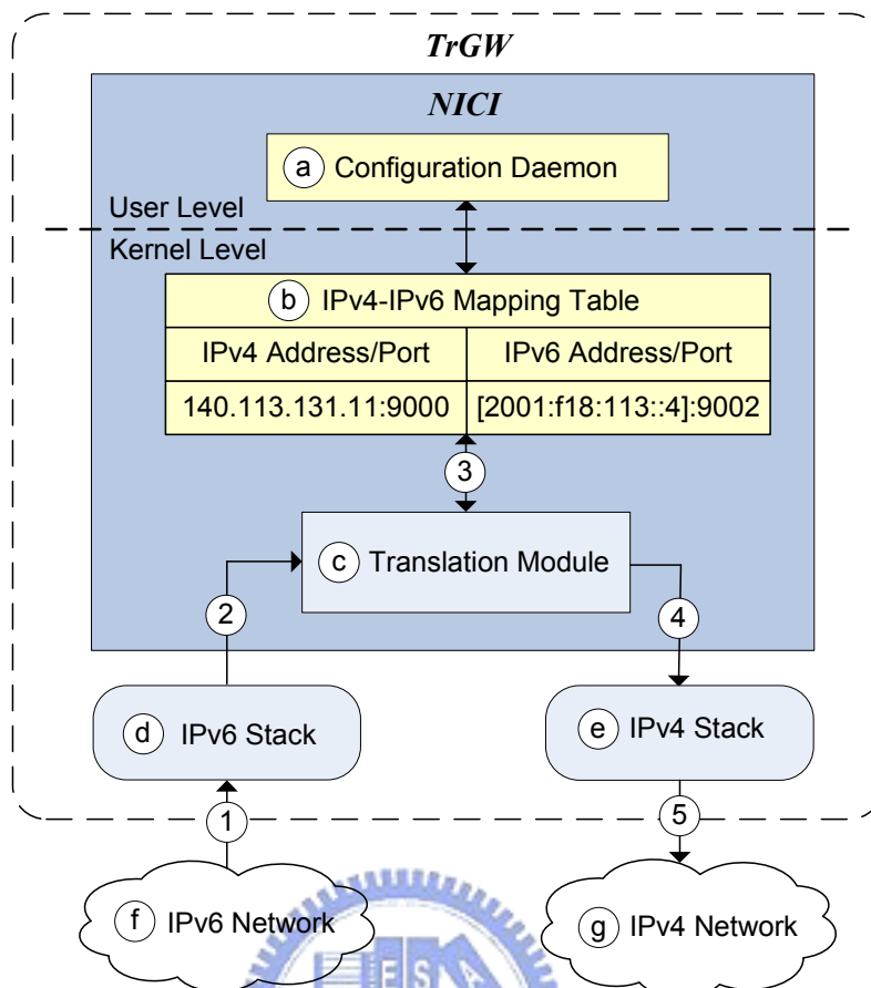
Fig. 6. NICI-TrGW Architecture
