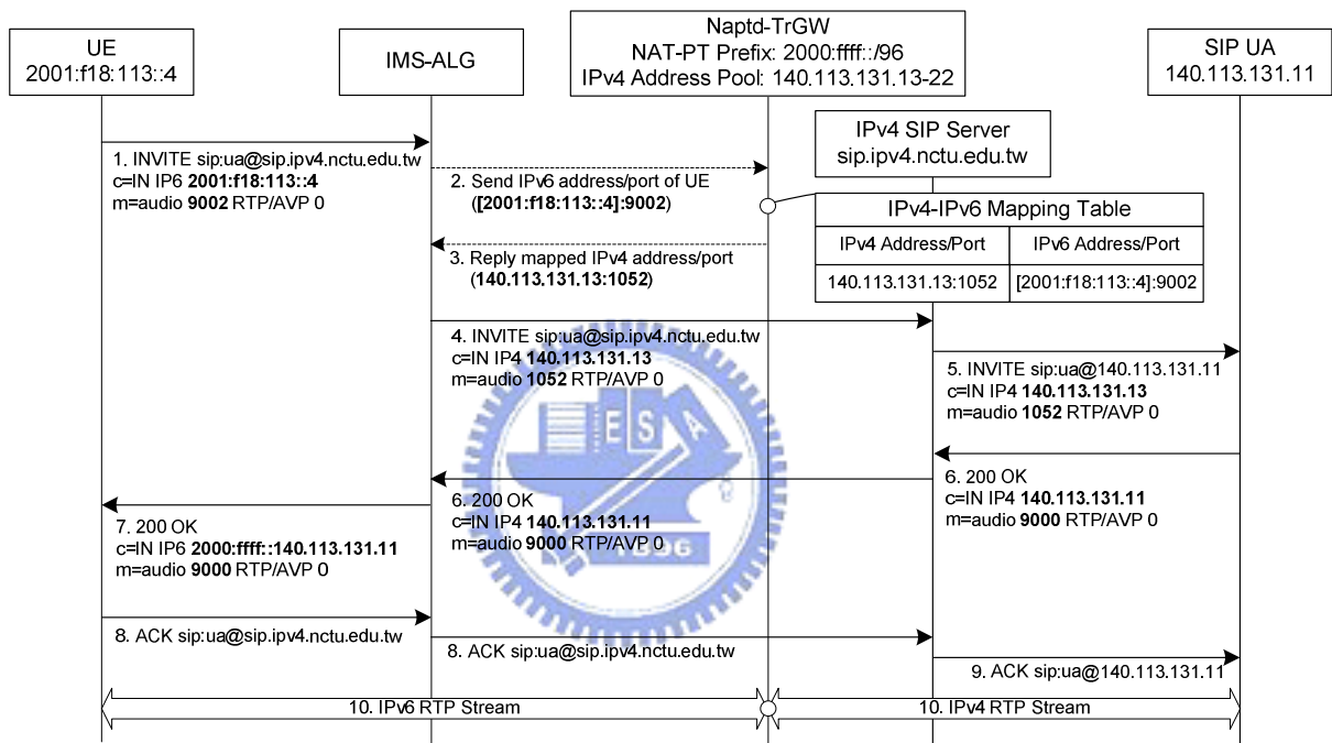
Fig. 2. SIP message flow with Napt-d-TrGW
