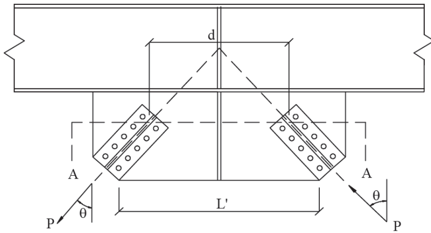
(a) Gusset Plate Subjected to Force P
