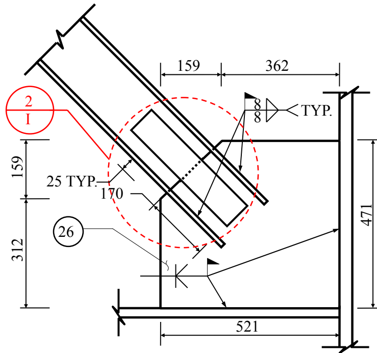
Unit: mm Specimen RGP Gusset Detail
