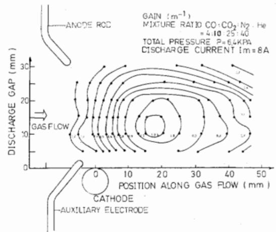
Fig. 10. Contours of constant gain in the discharge region.
