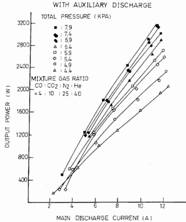
Fig. 6. The laser power versus discharge current with an auxiliary discharge.
