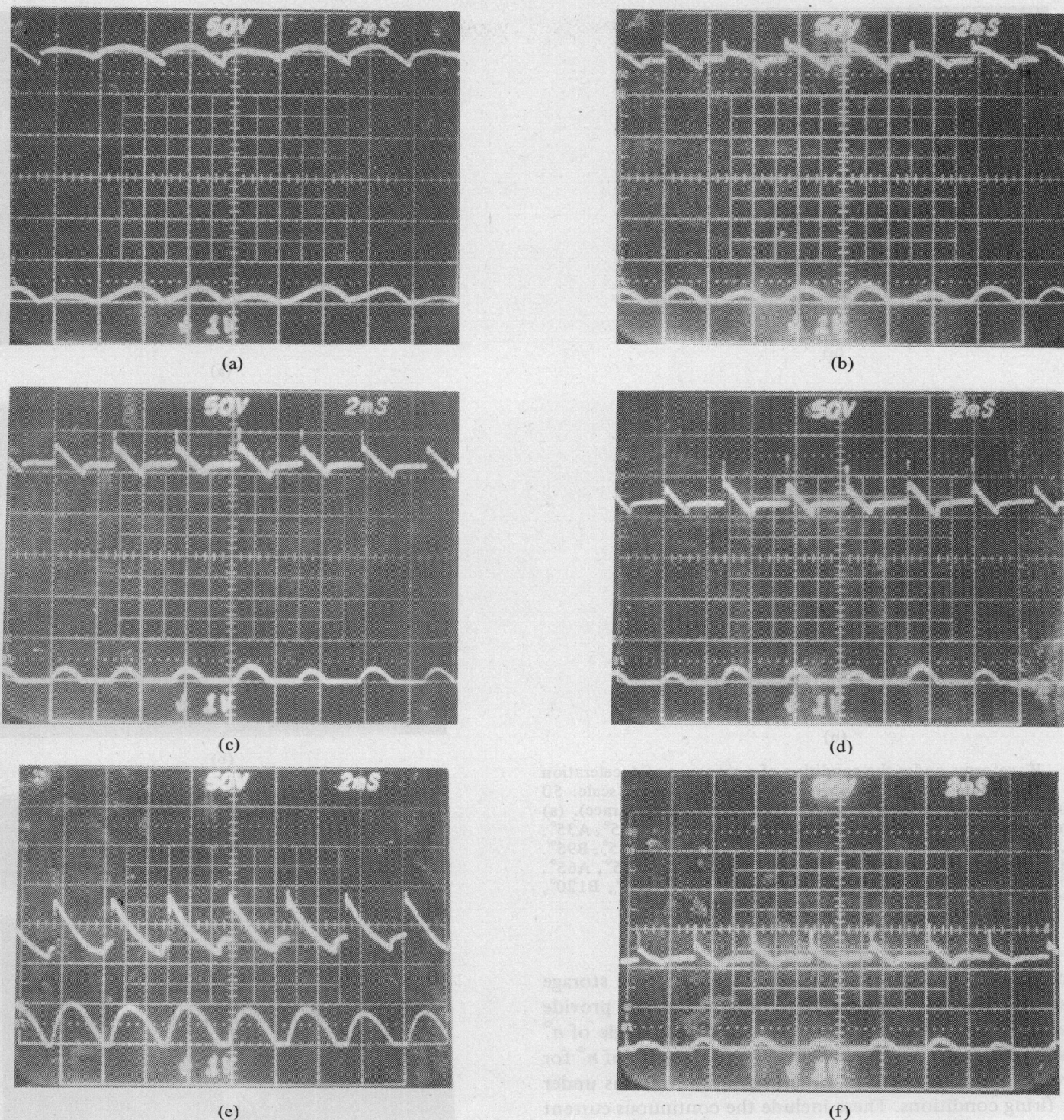
Fig. 11. Waveforms of armature voltage and current, horizontal scale: 2 ms/div; voltage scale: 50 V/div (upper trace); current scale: amp/div (lower trace). (a) Firing angle = A5^\circ . (b) Firing angle = A35^\circ . (c) Firing angle = A65^\circ . (d) Firing angle = A95^\circ . (e) Firing angle = A125^\circ . (f) Firing angle = A155^\circ .
