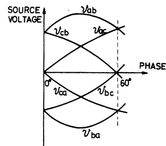
Fig. 7. Power source voltage signals.
