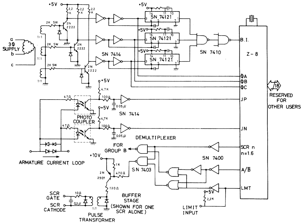
Fig. 2. Firing circuit.
