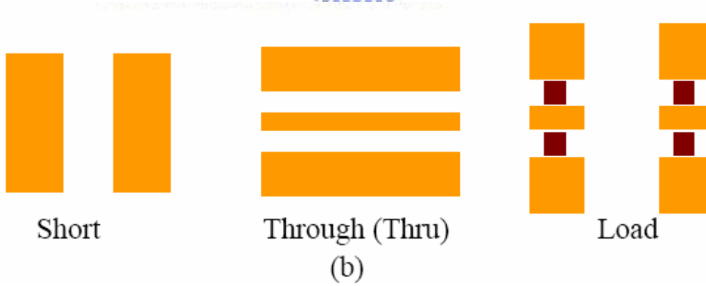
Fig. 3.19 Short, through and loads for the calibration
