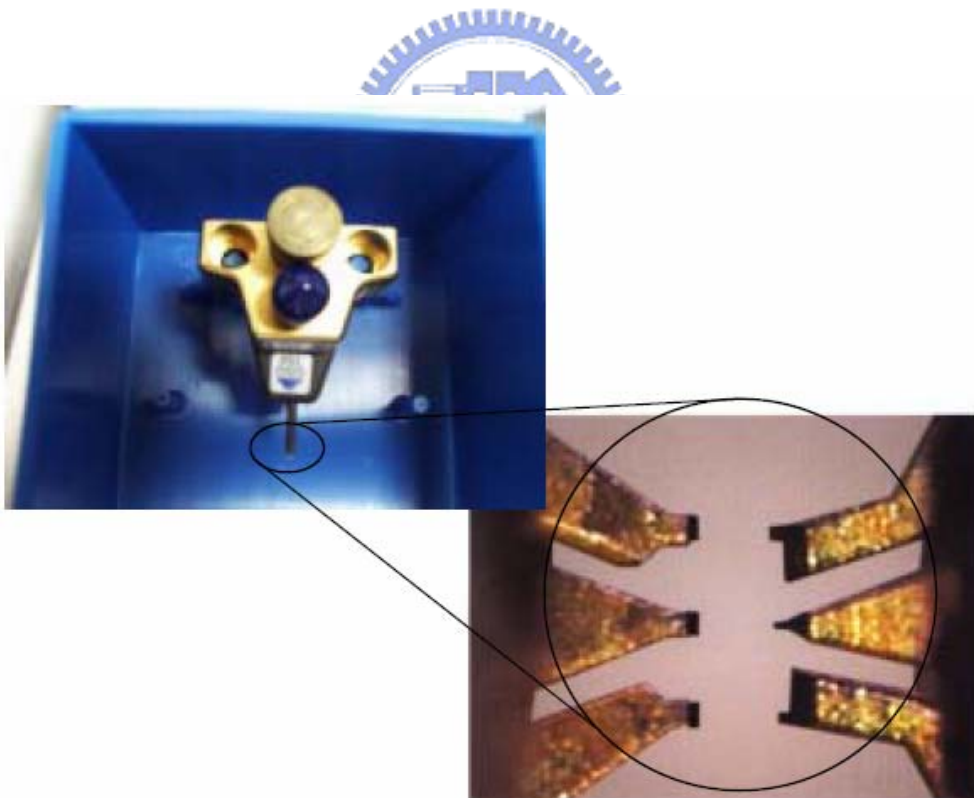
Fig. 3.17 CGS probe tips for the microwave measurement
