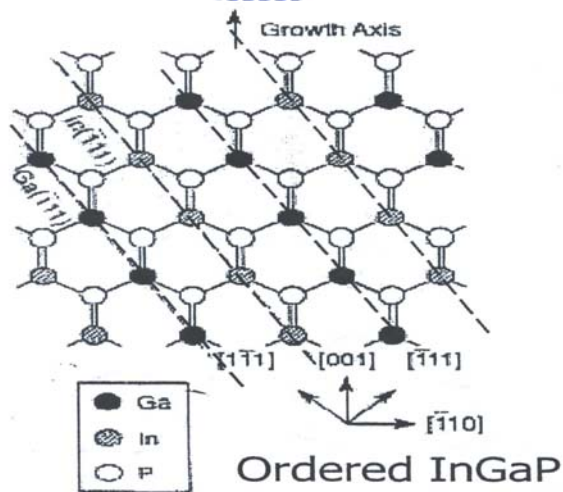
Fig 3.1b The 2-D diagram of the ordering InGaP.
