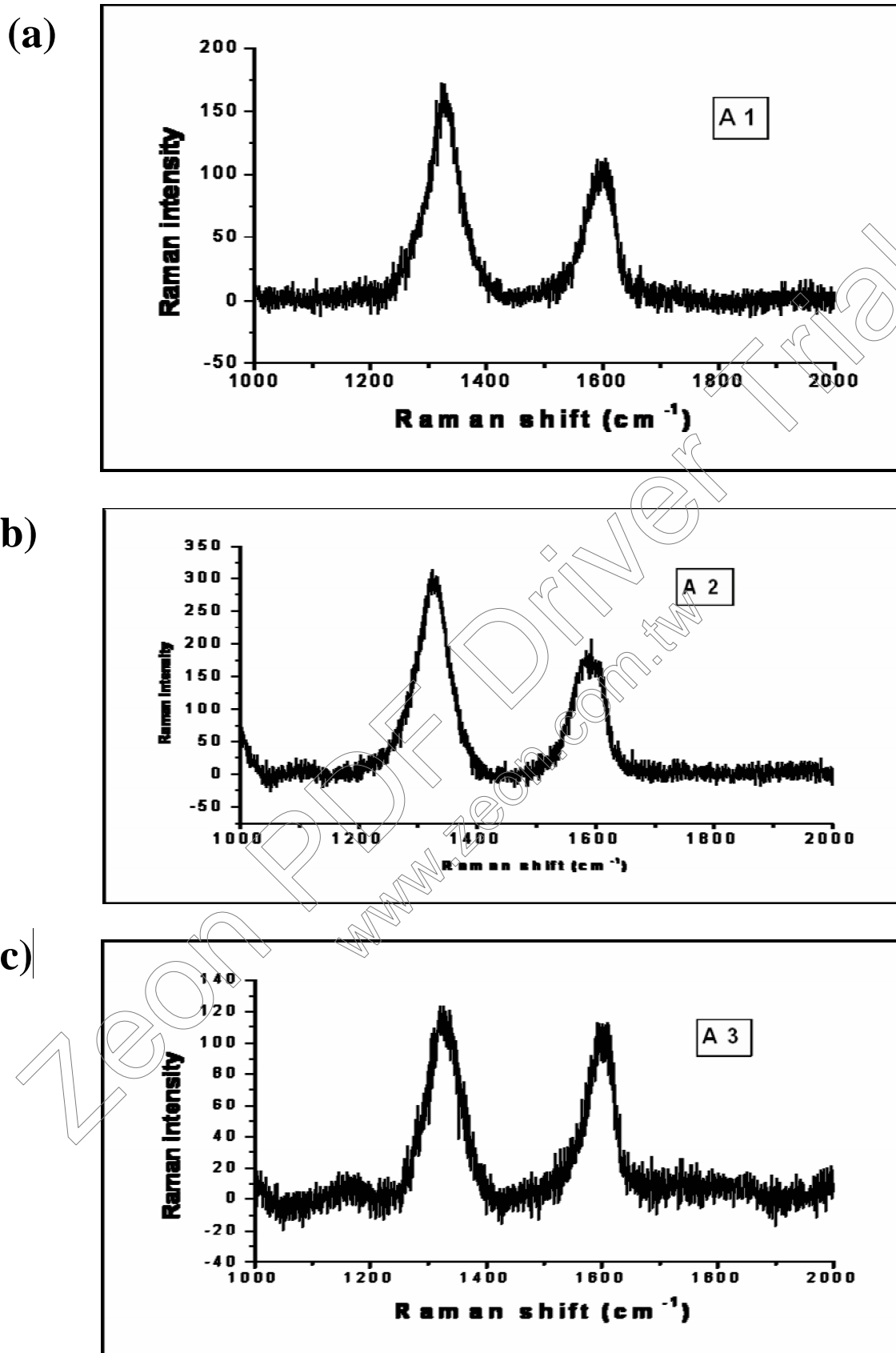
Fig. 4-16 Raman spectra of 100 nm Co-assisted CNTs grown with different \text{H}_2/\text{CH}_4 ratio (sccm/sccm) (a) 10/20 (b) 10/10 (c) 20/10.
