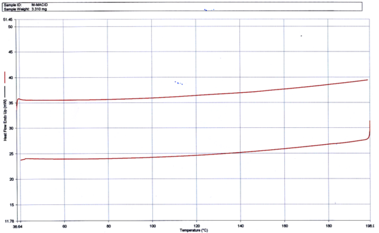
附圖 29. PDMB3OC10MA-m-MC 10 BA third heating-cooling 之 DSC 圖
