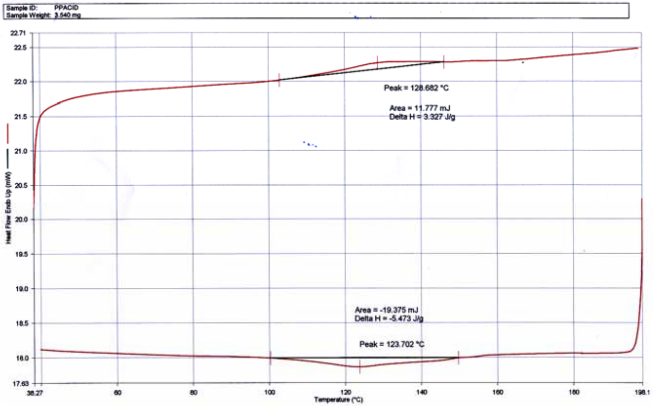
附圖 32. PDMB3OC10MA-p-PC 10 BA third heating-cooling 之 DSC 圖
