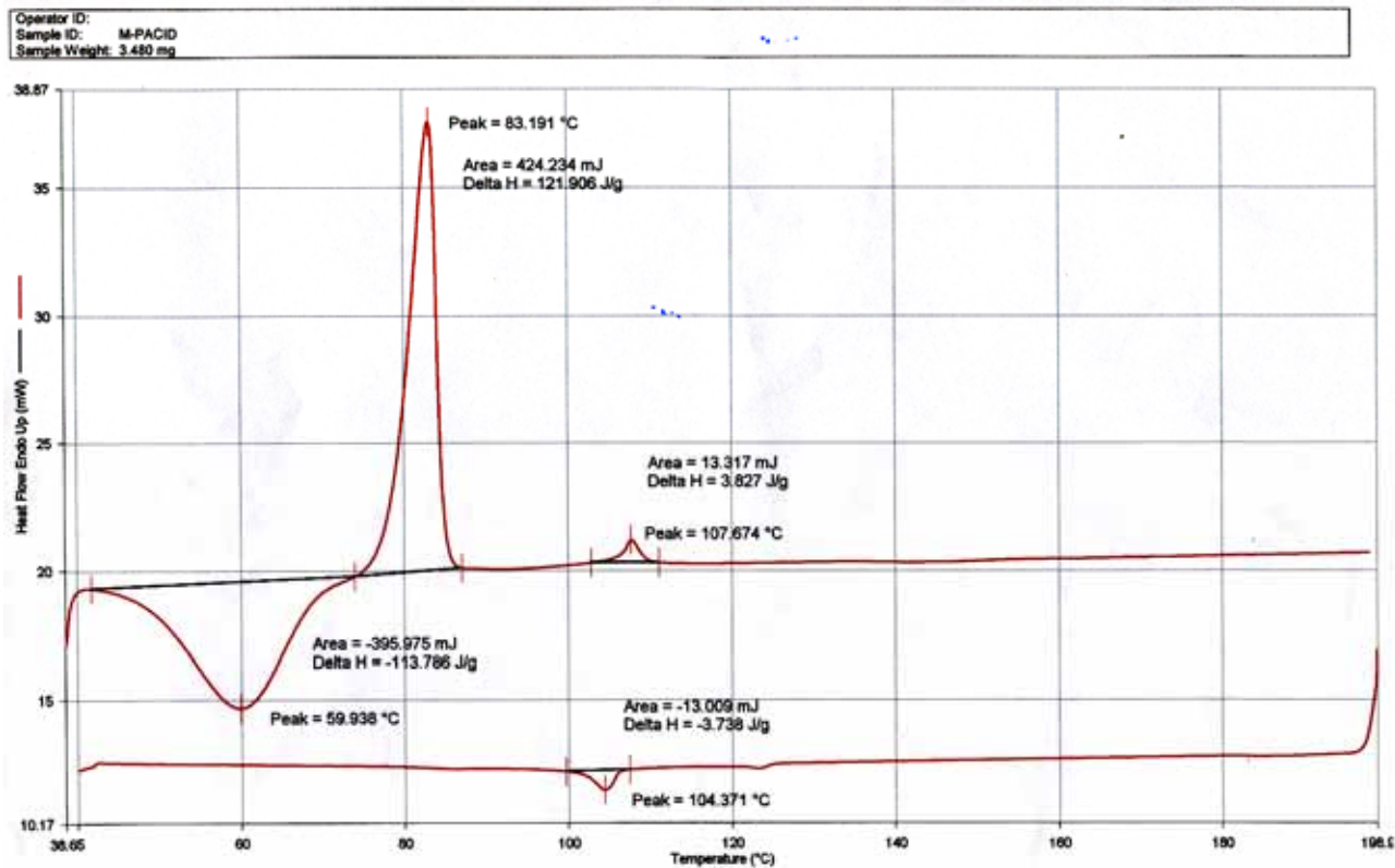
附圖 26. PDMB3OC10MA-p-MC 10 BA third heating-cooling 之 DSC 圖
