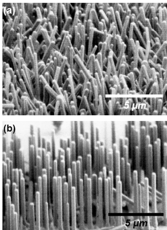
Figure 6.3 FESEM photographs for (a) Au and (b) Cu catalyzed ZnO nanowires synthesized on p-type Si (100) substrate with adopting CGFP method.
