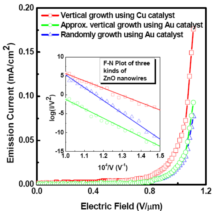
Figure 6.8 Field emission characteristics of the ZnO nanowires grown on p-type Si substrates. The inset reveals the F-N plots of the ZnO nanowires.
