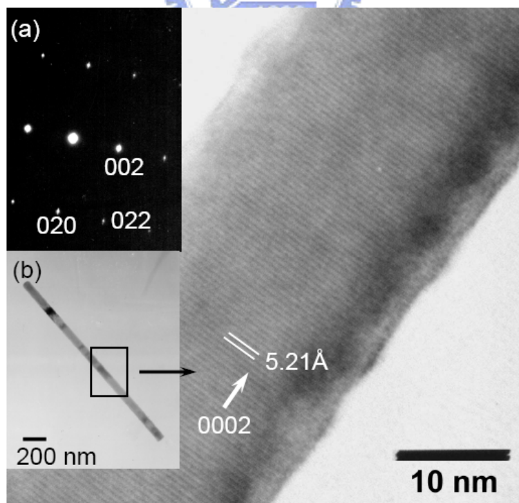
Figure 6.5 HRTEM image of Cu catalyzed ZnO nanowires. The selected area electron diffraction (SAED) pattern is shown in inset (a), while bright view image for side wall of the ZnO nanowires, is indicated in inset (b).
