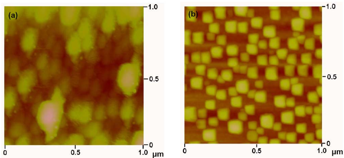
Figure 6.1 AFM images of the (a) Au and (b) Cu thin film surface after heating process.
