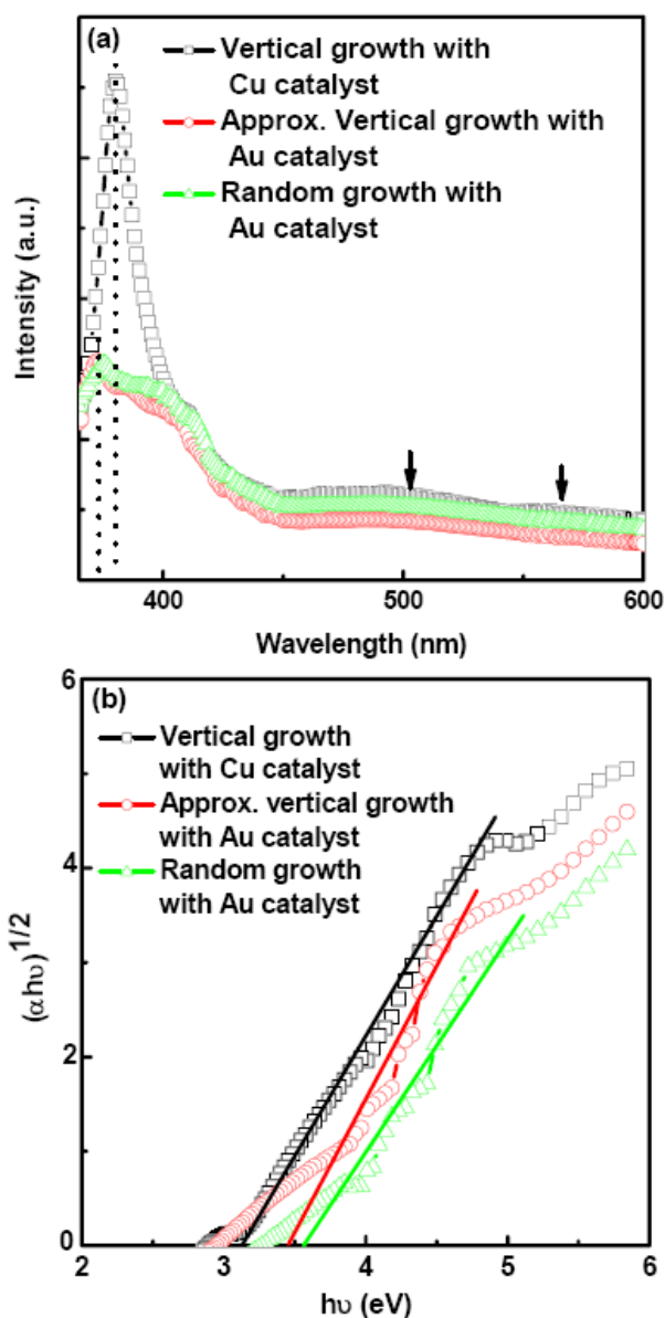
Figure 6.7 (a) PL spectra of the ZnO nanowires grown on the p-type Si substrate. (b) Tauc's plot of the ZnO nanowires grown on the P-type Si Substrate.
