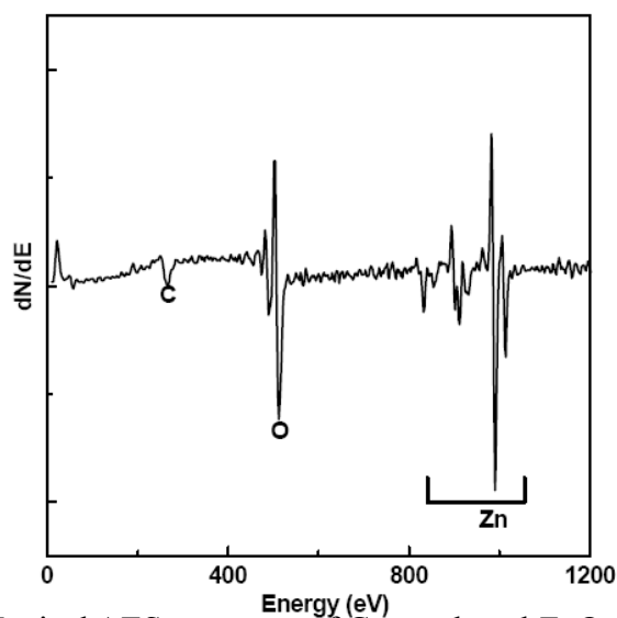
Figure 6.6 Typical AES spectrum of Cu catalyzed ZnO nanowires.
