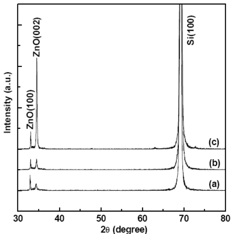
Figure 6.4 XRD patterns of ZnO nanowires synthesized with (a) Au as the catalyst, (b) Au as the catalyst by CGFP method, and (c) Cu as the catalyst by CGFP method.
