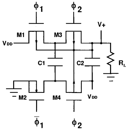
Fig. 1. A CMOS voltage doubling charge pump circuit.
