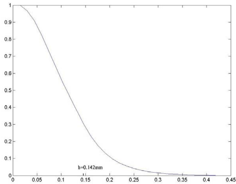
Fig.3(b) z -direction with \mu=-0.2004
