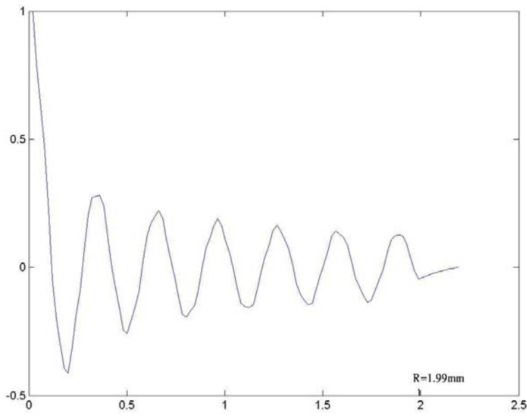
Fig.3(a) \rho -direction with \mu=-0.2004
