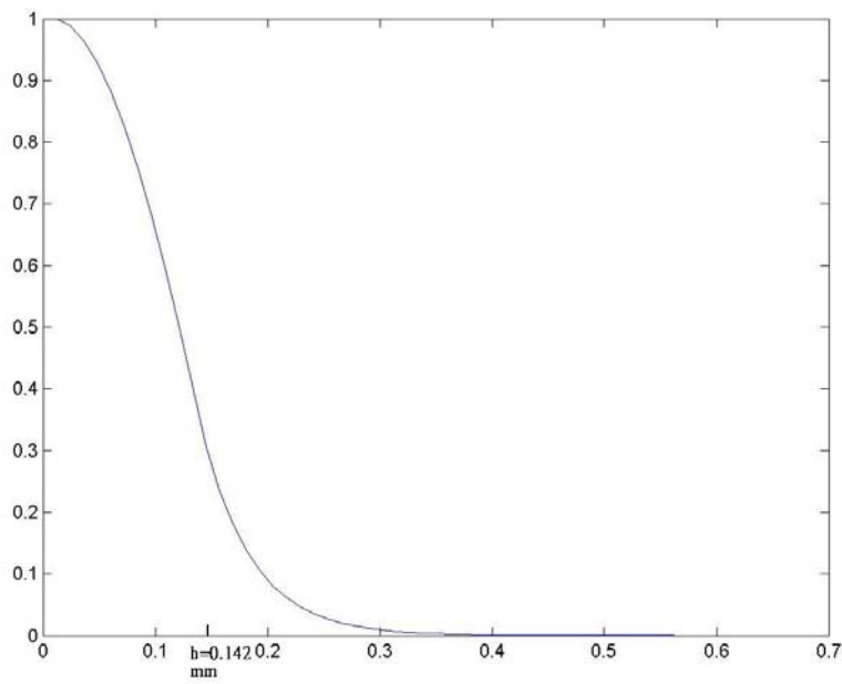
Fig.2(b) z-direction with \mu=-0.1595
