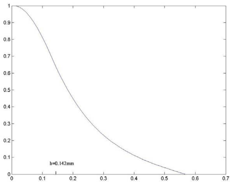
Fig.7(b) z-direction with \mu=-0.9710
