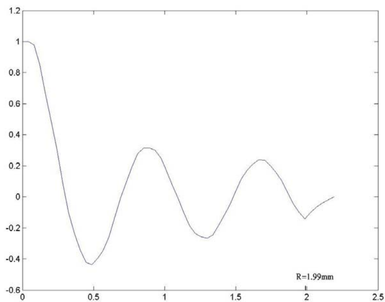
Fig.4(a) \rho -direction with \mu=-0.2875
