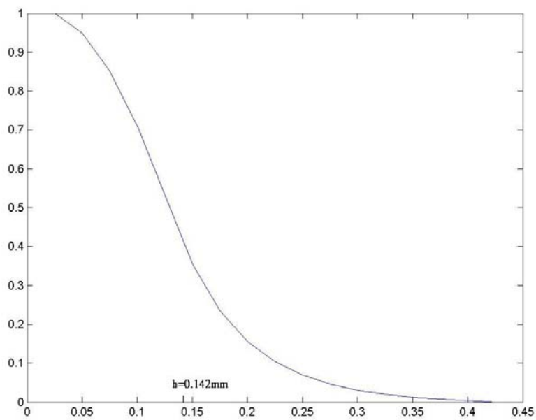
Fig.6(b) z-direction with \mu=-0.2994
