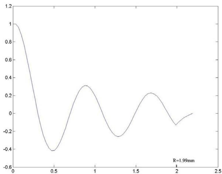
Fig.6(a) \rho -direction with \mu=-0.2994
