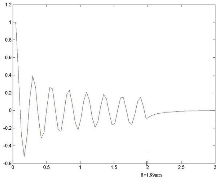
Fig.2(a) \rho -direction with \mu=-0.1595
