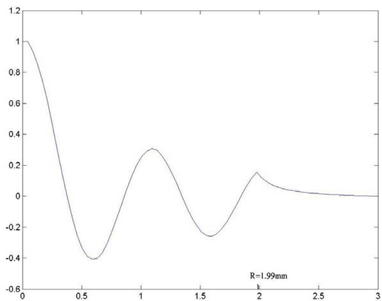
Fig.7(a) \rho -direction with \mu=-0.9710
