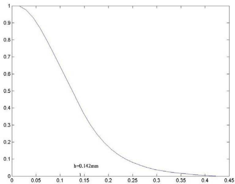
Fig.5(b) z -direction with \mu=-0.2973
