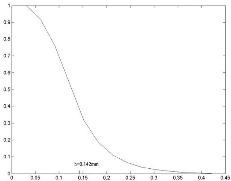
Fig.4(b) z -direction with \mu=-0.2875
