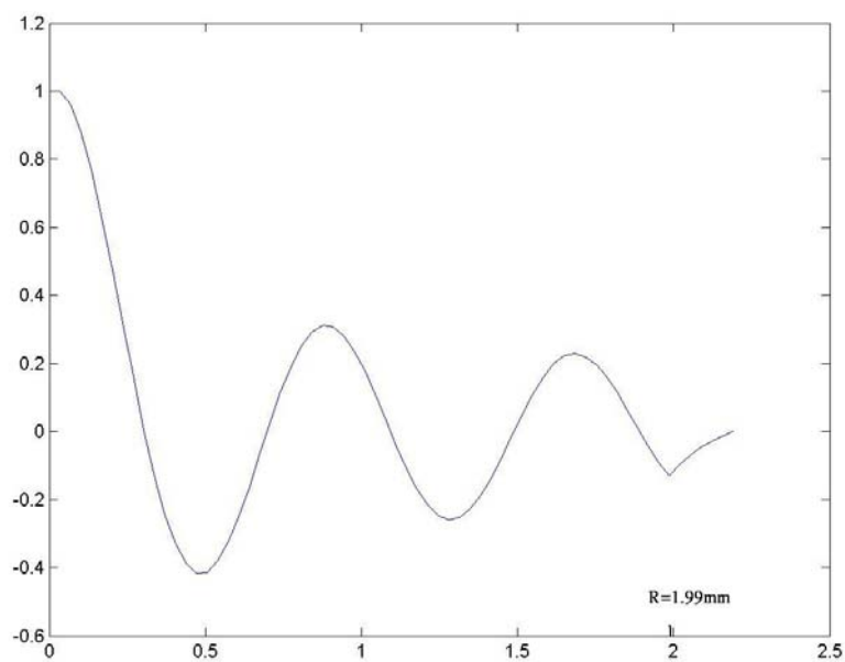
Fig.5(a) \rho -direction with \mu=-0.2973
