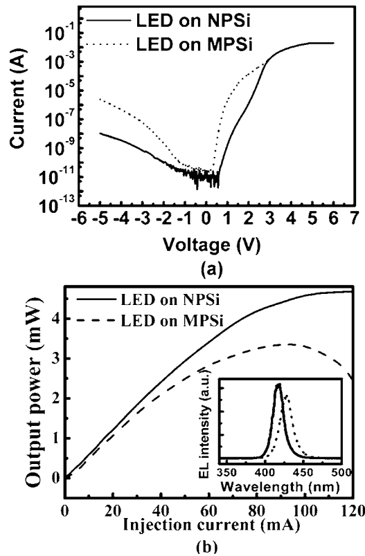
FIG. 4. (a) The I-V characteristics. (b) The L-I curves. The inset is the comparison of EL spectra at 20 mA injection current.
