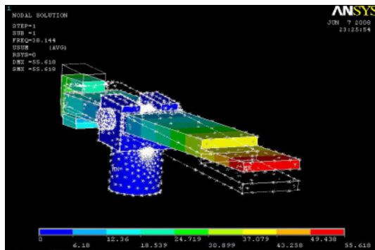
Fig. 6. (Color online) Mode I cantilever: 38 Hz.
