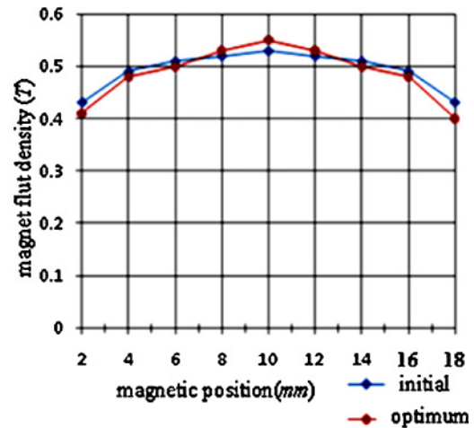
Fig. 18. (Color online) Comparison of magnetic flux density between initial design and optimum design.
