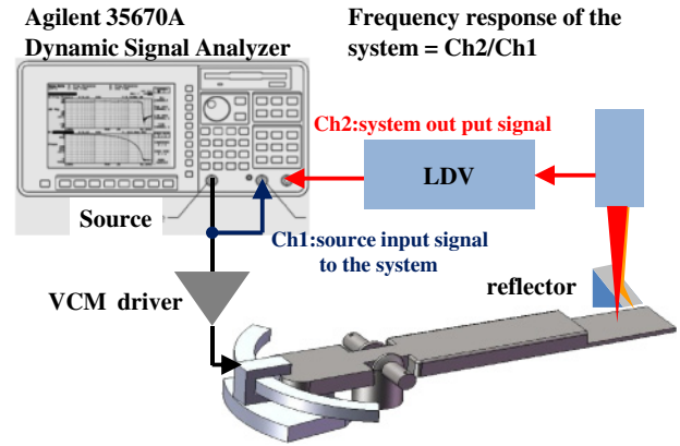
Fig. 11. (Color online) Dynamic response experimental apparatus.
