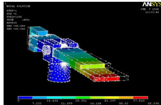
Fig. 7. (Color online) Mode II first bending: 1285.6 Hz.
