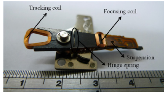
Fig. 3. (Color online) DataPlay's swing arm actuator.
