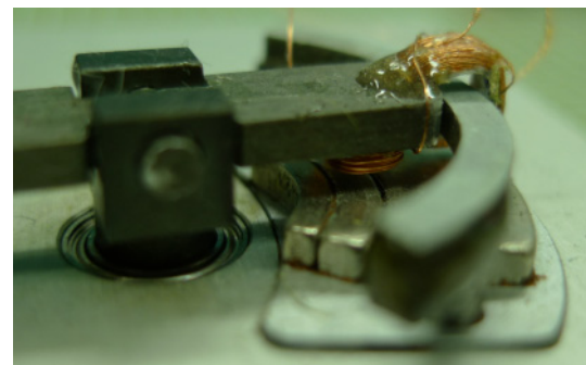
Fig. 8. (Color online) Lateral view of MSMA magnets.
