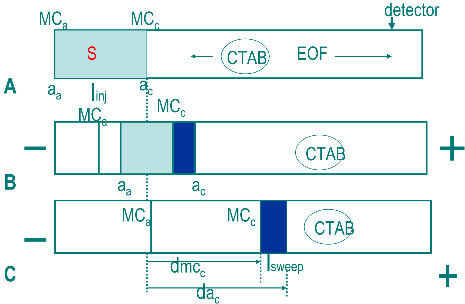
Fig.6-1 Schematic diagram of sweeping under CTAB micelle.
