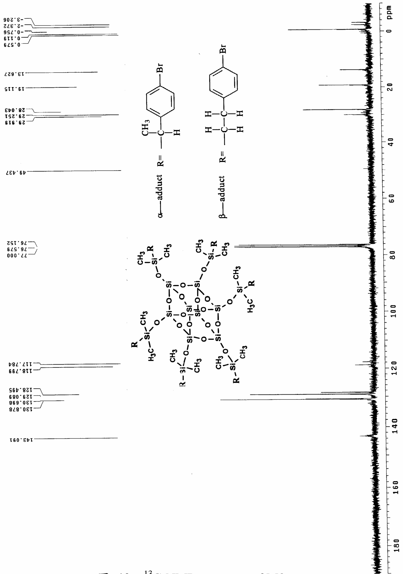
附圖. 10 ^{13}\text{C} -NMR spectrum of M3
