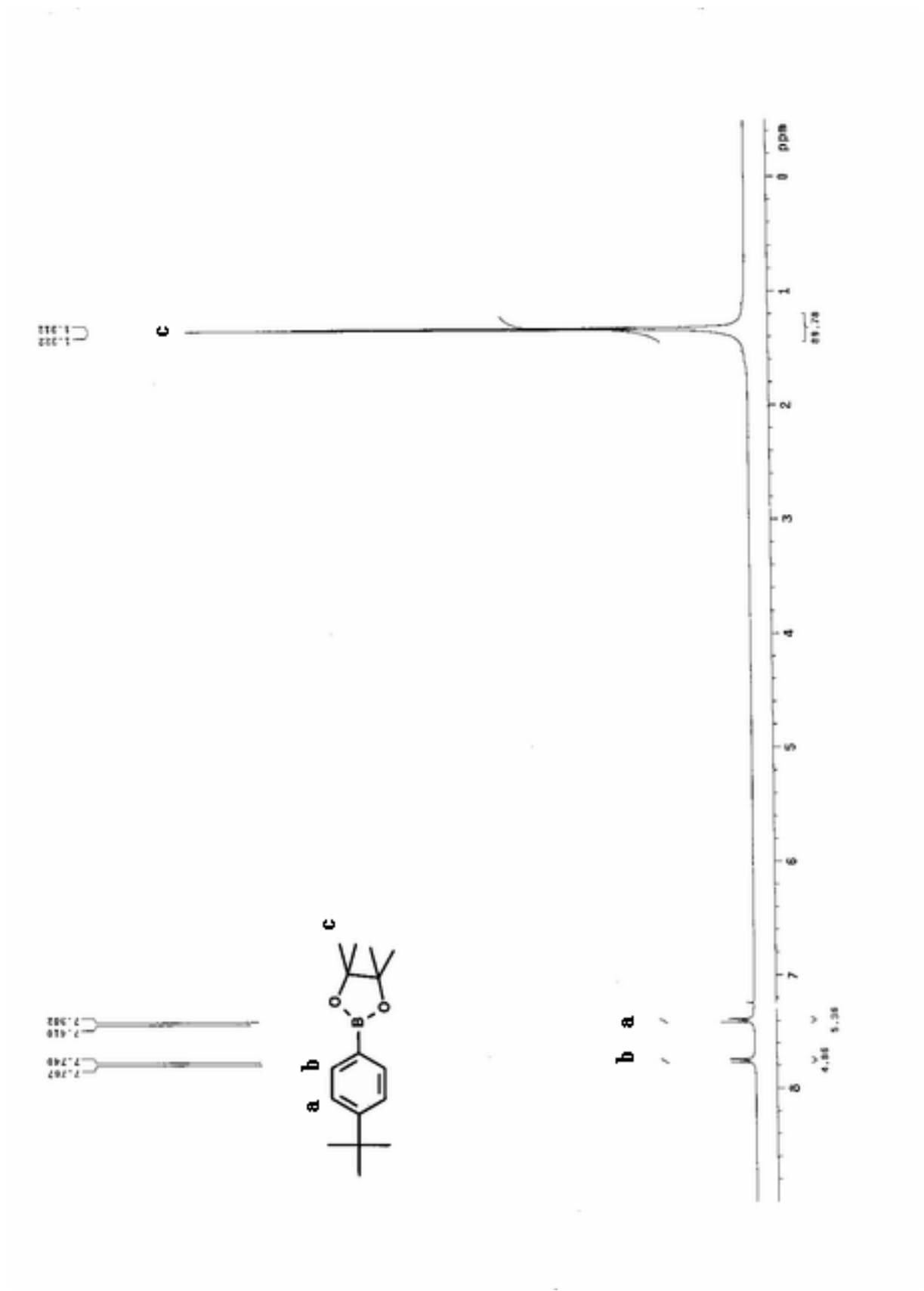
附圖.7 ^1\text{H-NMR} spectrum of M7
