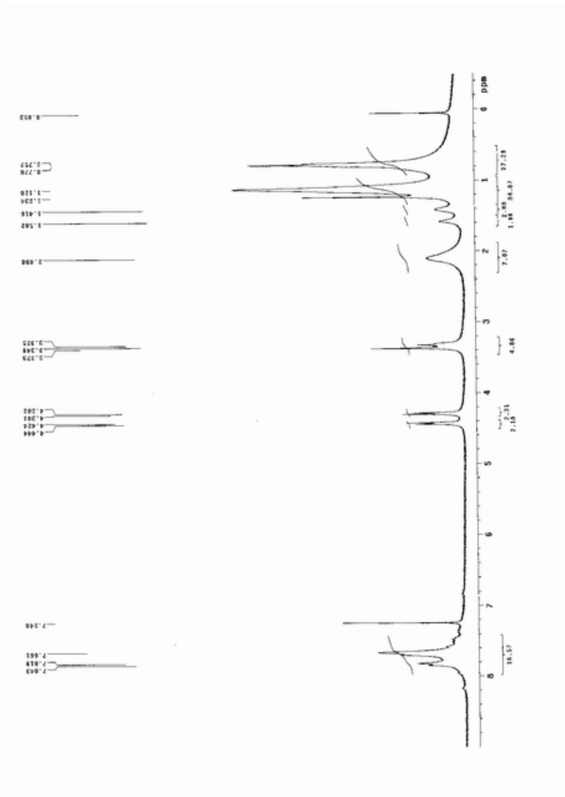
附圖.26 ^1\text{H-NMR} spectrum of P5
