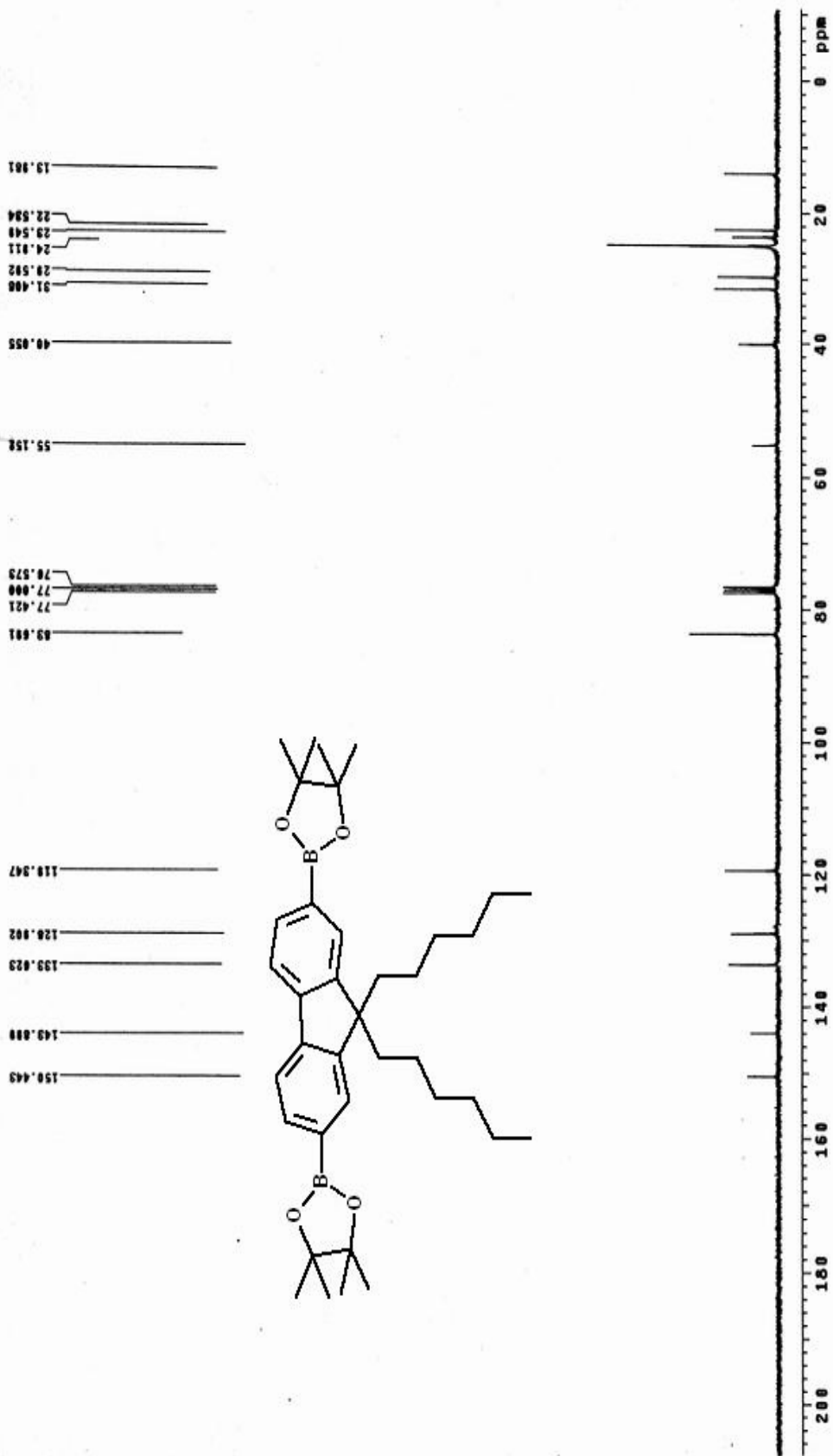
附圖.10 13 C-NMR spectrum of M3
