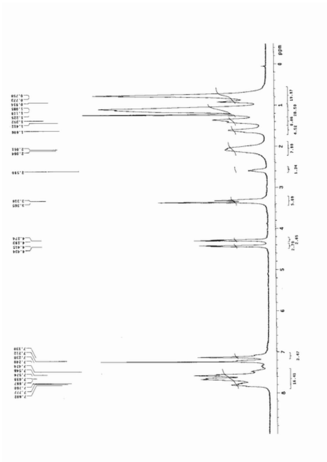
附圖.22 ^1\text{H-NMR} spectrum of P1
