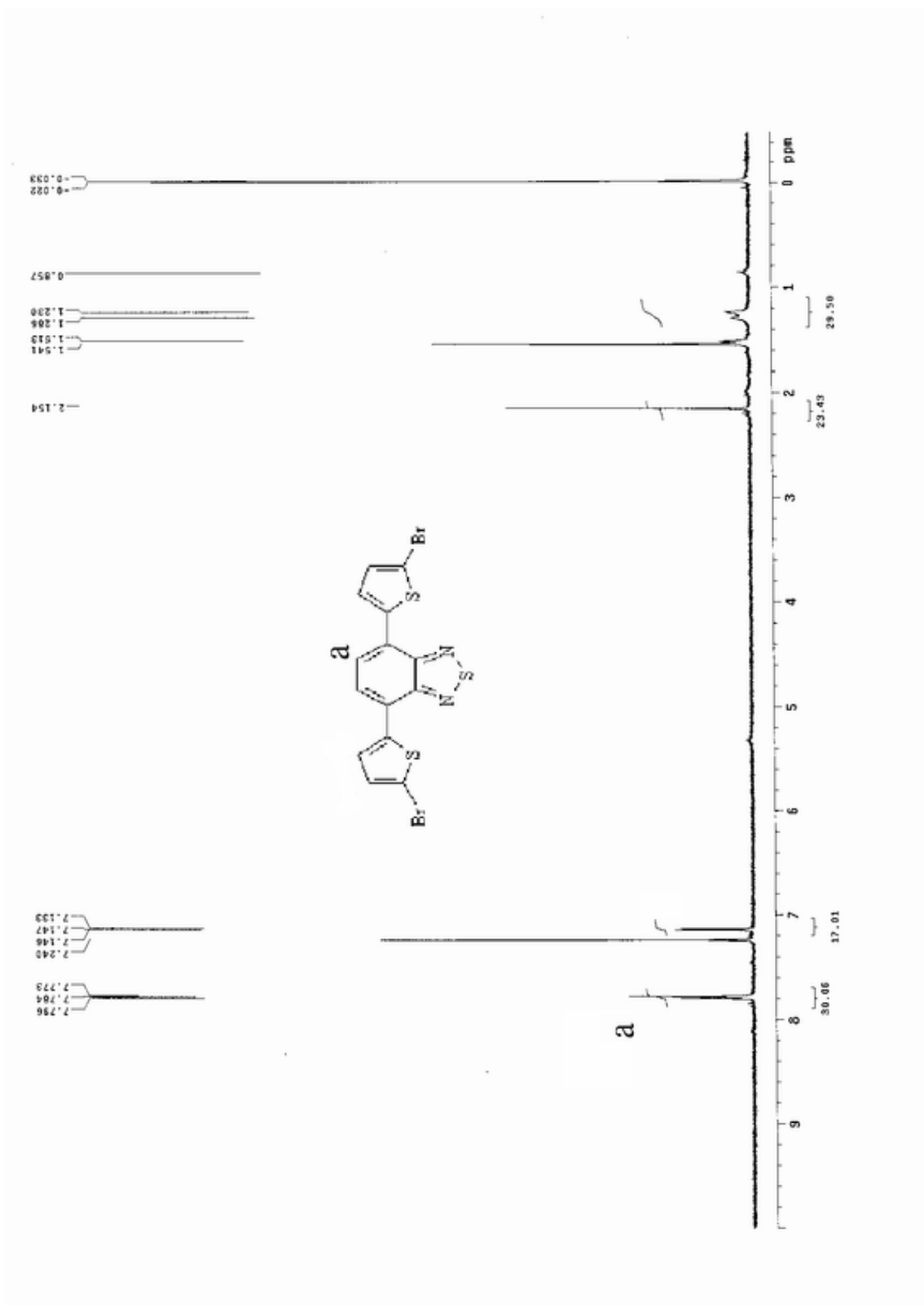
附圖.6 ^1\text{H-NMR} spectrum of M6
