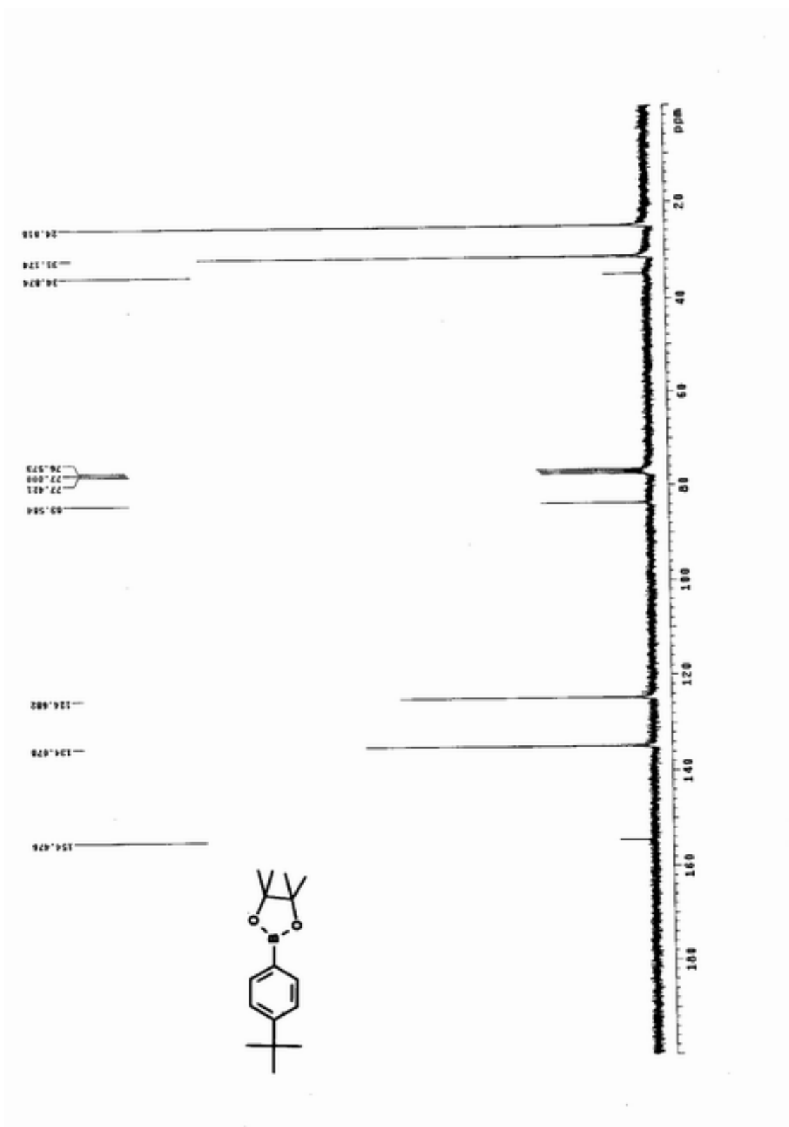
附圖.14 ^{13}\text{C} -NMR spectrum of M7
