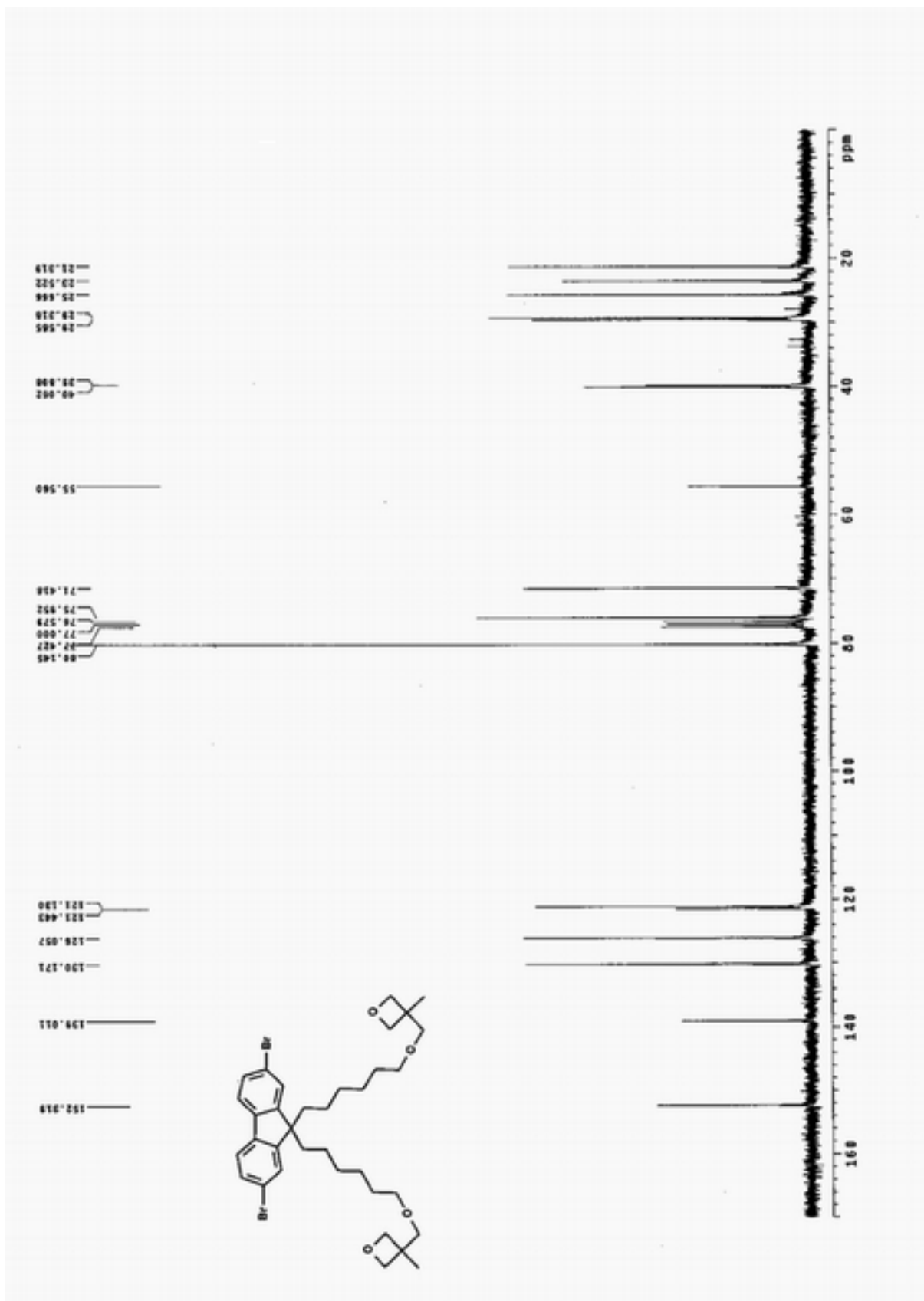
附圖.8 ^{13}\text{C} -NMR spectrum of M1
