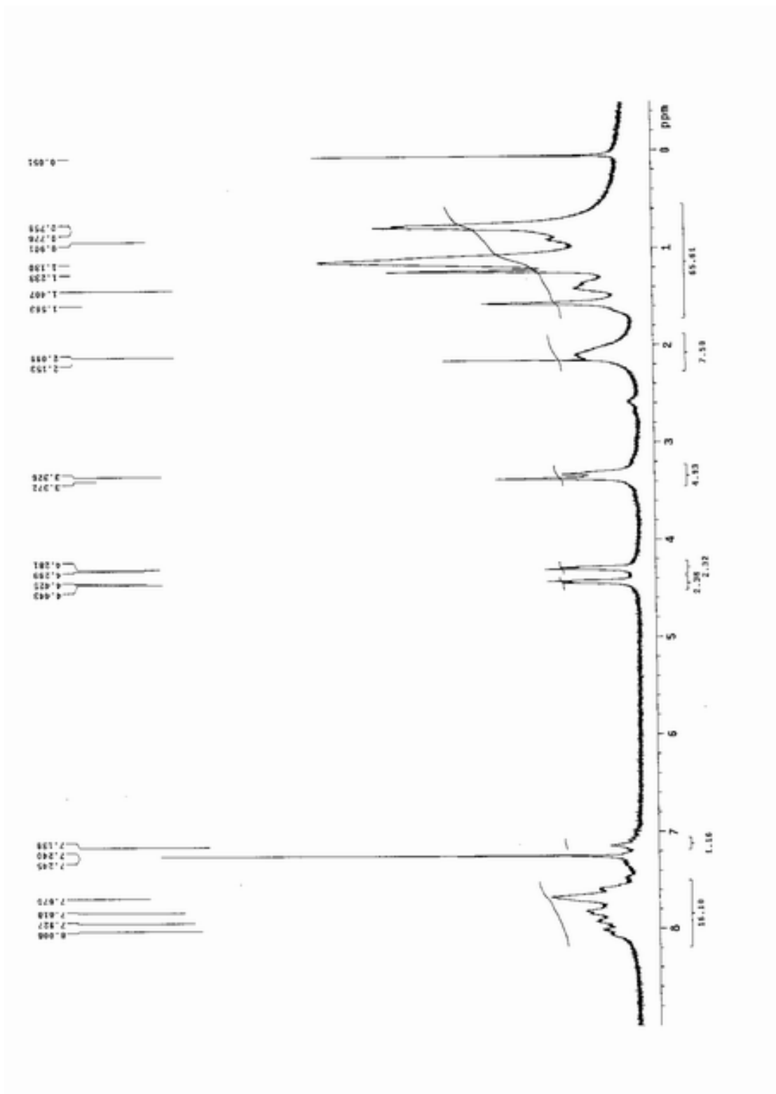
附圖.25 ^1\text{H-NMR} spectrum of P4
