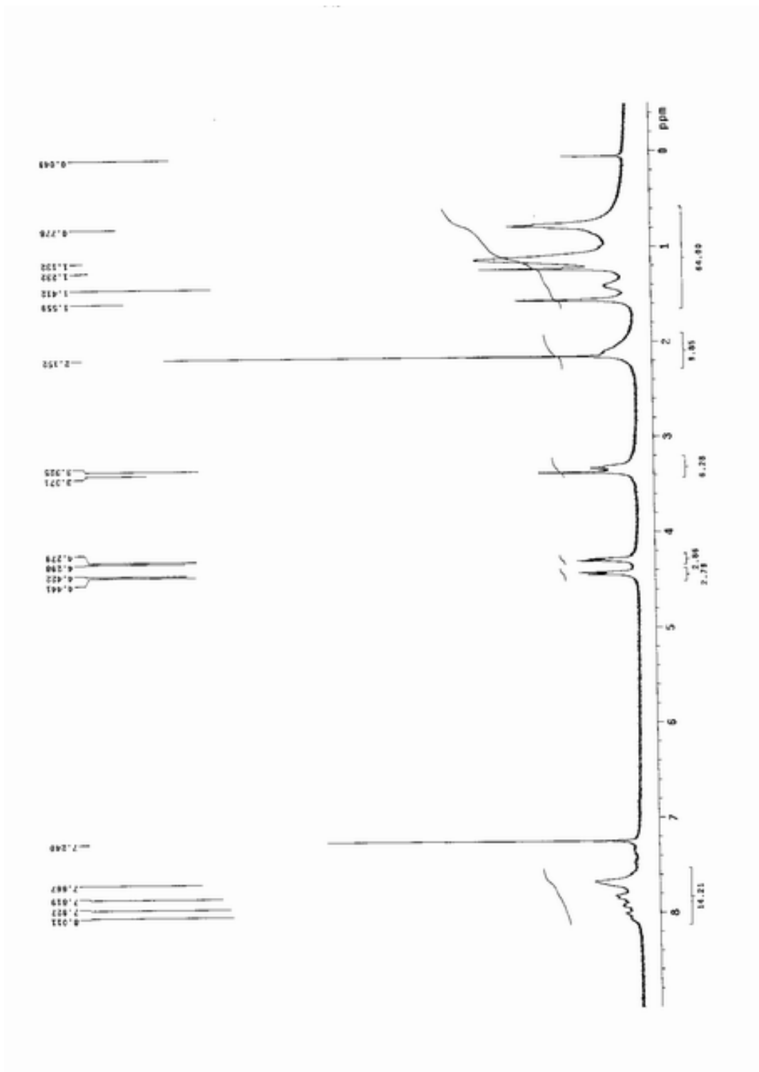
附圖.24 ^1\text{H-NMR} spectrum of P3
