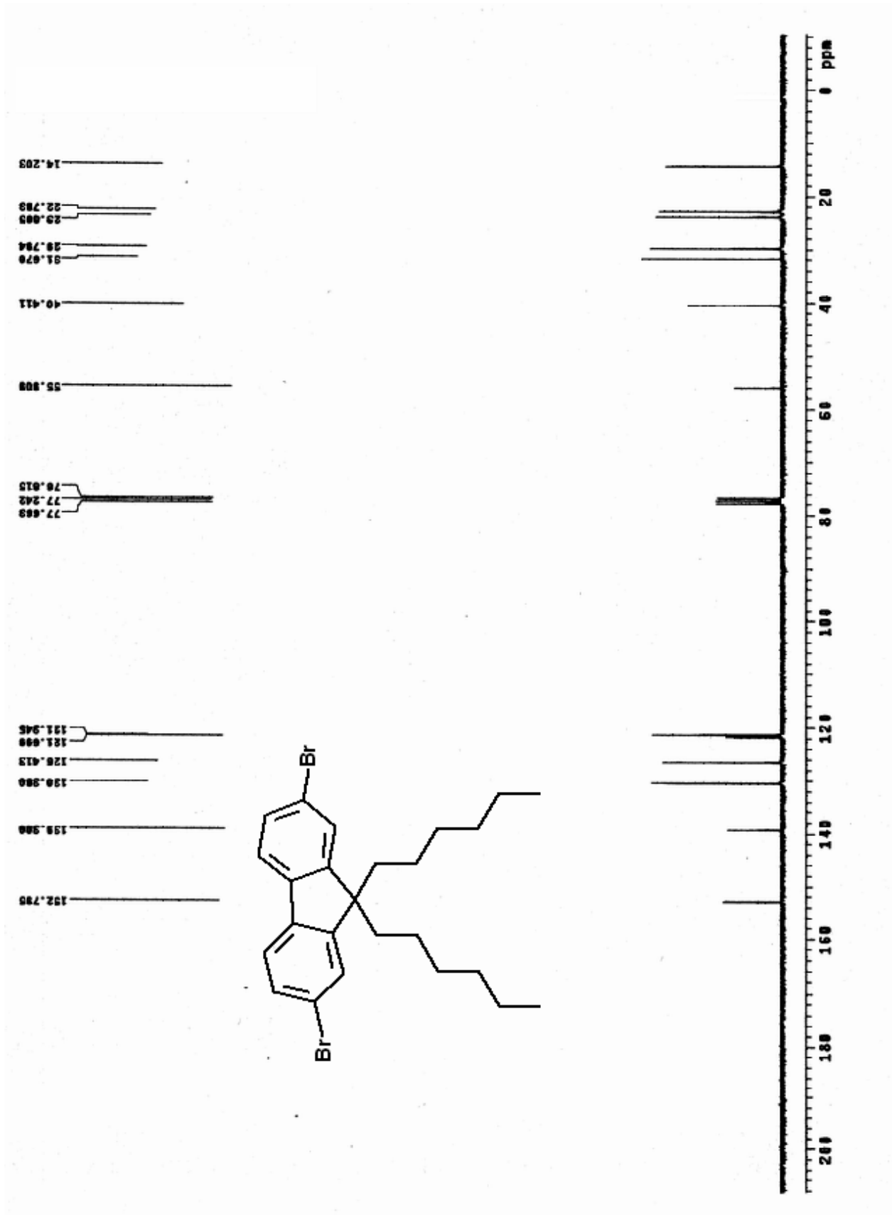
附圖.9 ^{13}\text{C} -NMR spectrum of M2
