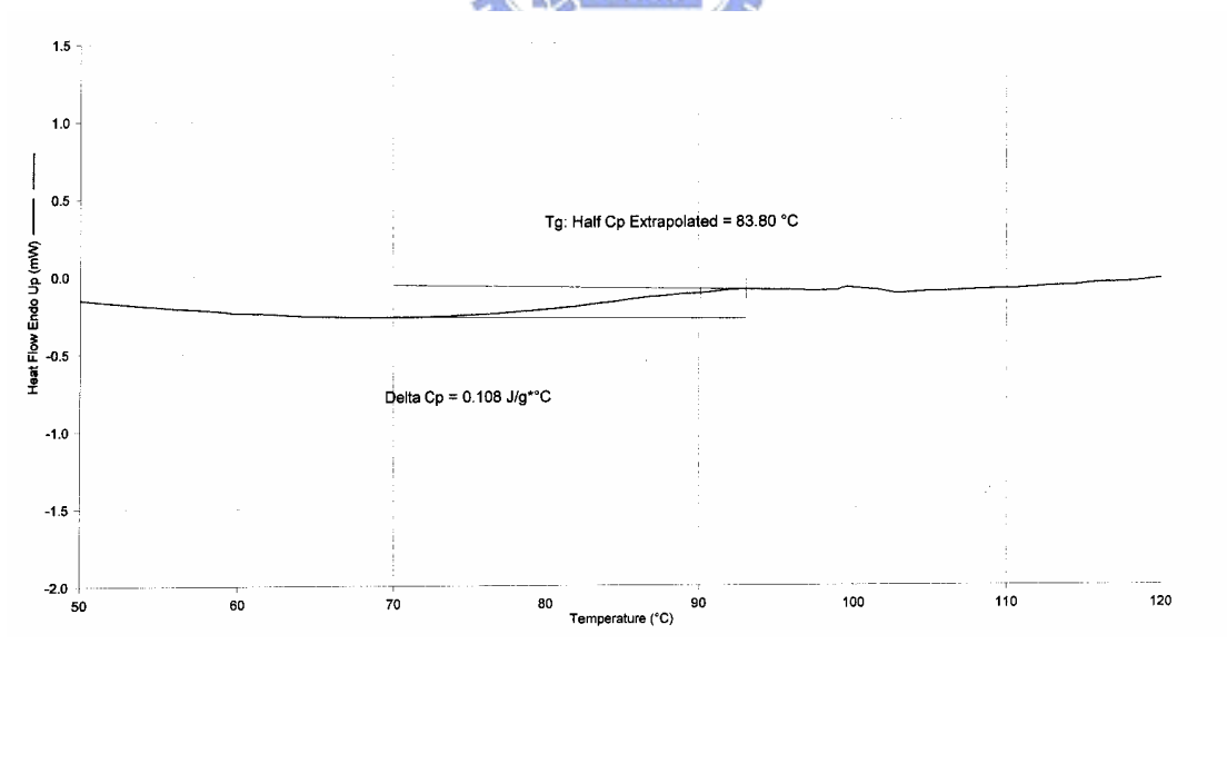
附圖.29 (a)TGA (b)DSC thermogram of P1
