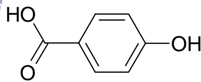
p -Hydroxybenzoic acid
