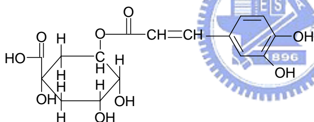
Chlorogenic acid
