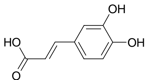
Caffeic acid
