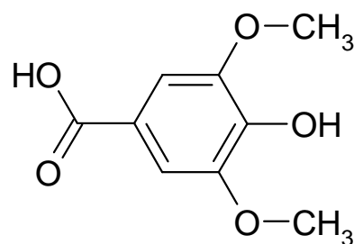
Syringic acid
