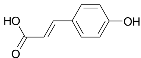
p -Coumaric acid
