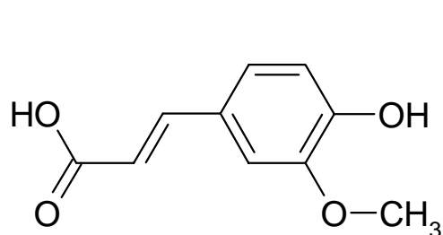
Ferulic acid
