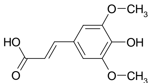
Sinapic acid
