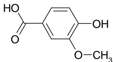
Vanillic acid
