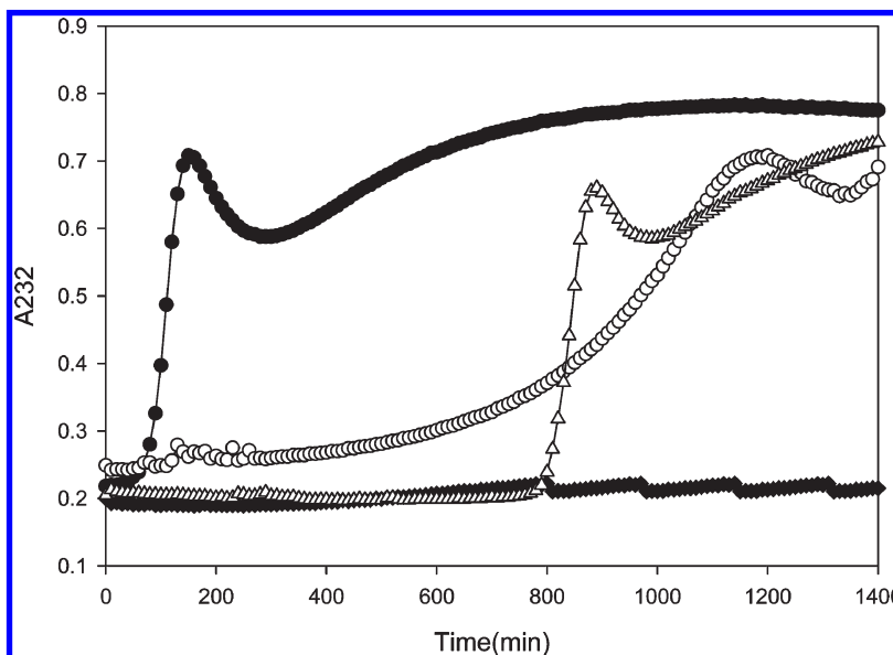
Figure 4. Effect of the peptide fraction from APWP on the \text{Cu}^{2+} -induced oxidation of human low-density lipoprotein (LDL): (●) PBS buffer; (△) the peptides 1.52 \mu\text{g/mL} ; (◆) no \text{Cu}^{2+} ; (○) Trolox 10 \mu\text{g/mL} .
