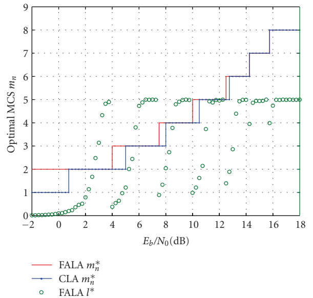
FIGURE 6: The FALA table \mathbf{T} : optimal selections of the MCS scheme m_n^* (left axis) and the MPDU payload size l^* (right axis) versus the SNR value. The optimal MCS schemes with fixed MPDU payload size ( l = 5 KBytes) is also illustrated for comparison purpose.
