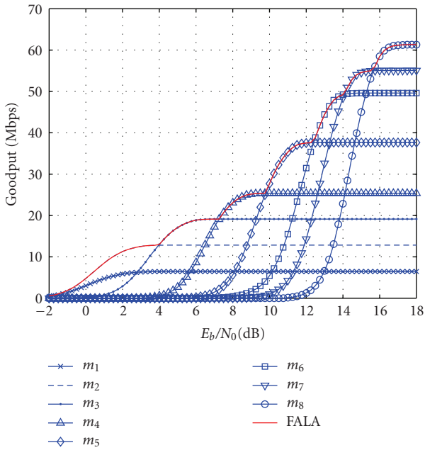
FIGURE 5: Maximal achievable goodput performance by adopting FALA algorithm and the eight MCS schemes.
