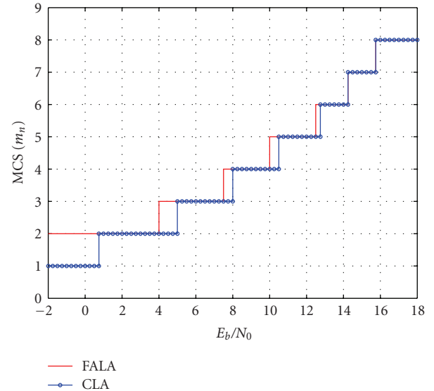
FIGURE 8: The corresponding MCS schemes versus SNR values adopted in the goodput comparison as in Figure 7.
