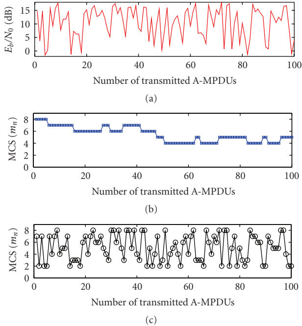
FIGURE 10: (a) the channel conditions within different transmission attempts generated by the two-state discrete Markov chain model with P_{b,g} = 0.7 . (b) the MCS scheme adopted by the ARF algorithm in every transmission attempt. (c) the MCS scheme exploited by the proposed FALA algorithm in every transmission attempt.
