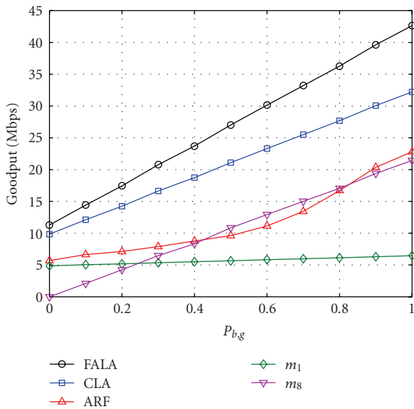
FIGURE 11: Performance comparison: average goodput versus channel variations with P_{b,g} from 0 to 1.
