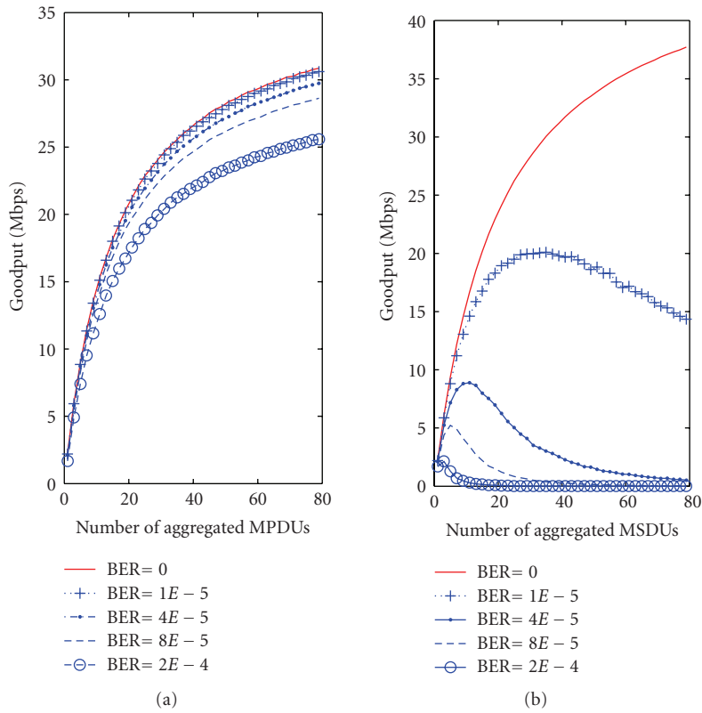
FIGURE 2: Goodput performance versus the number of aggregated MPDUs (a) and the number of aggregated MSDUs (b).
