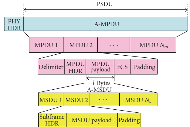
FIGURE 1: The schematic diagram of A-MPDU and A-MSDU frame formats.
