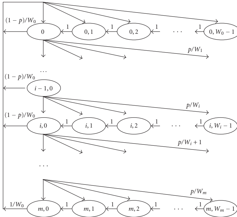
FIGURE 3: Two-dimensional Markov chain backoff model in consideration of packet collision and channel noises.
