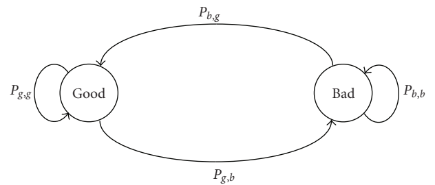
FIGURE 9: A two-state discrete Markov chain model for channel variations.
