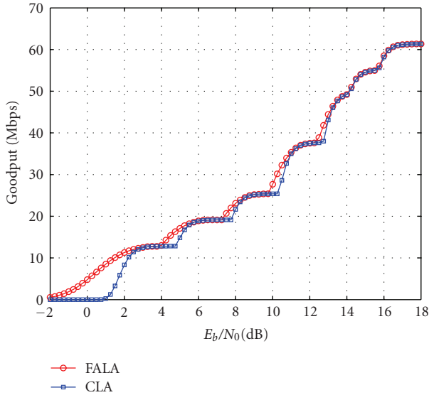
FIGURE 7: Performance comparison: goodput versus SNR value. The MPDU payload size for FALA algorithm l \in [10, 5000] , and MPDU payload size for CLA scheme l = 5000 bytes.
