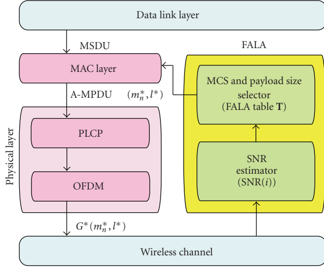
FIGURE 4: The system architecture for the proposed FALA algorithm.
