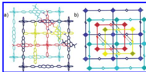
Figure 3. Simplified stacking diagrams of MAS-1 highlighting (a) the unique layer-to-layer \text{NH}\cdots\text{N} hydrogen bonds and (b) the distorted 6^4.8^2\text{-nbo} network topology.
