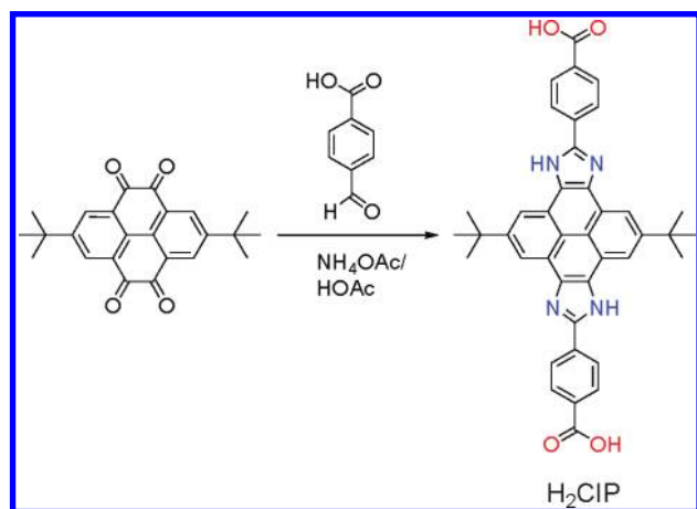
Scheme 1. Synthesis Route to the H 2 CIP Ligand
